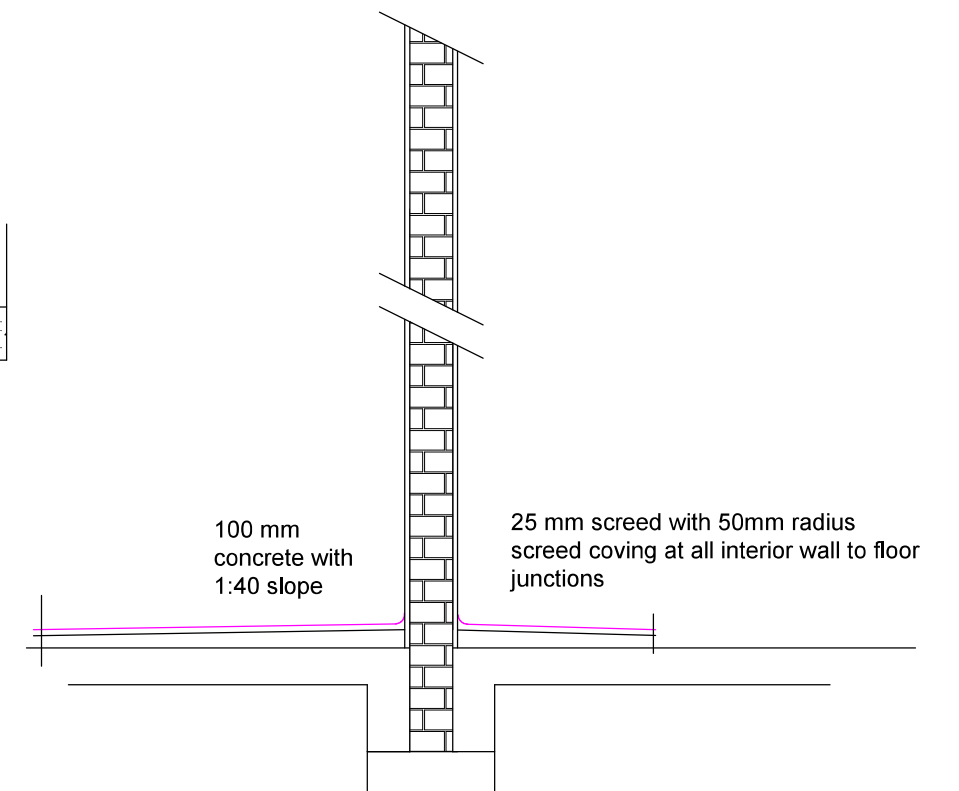
DETAIL A
