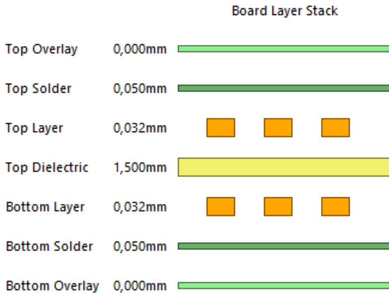
Figure 1: PCB Layer Stack Up Summary
