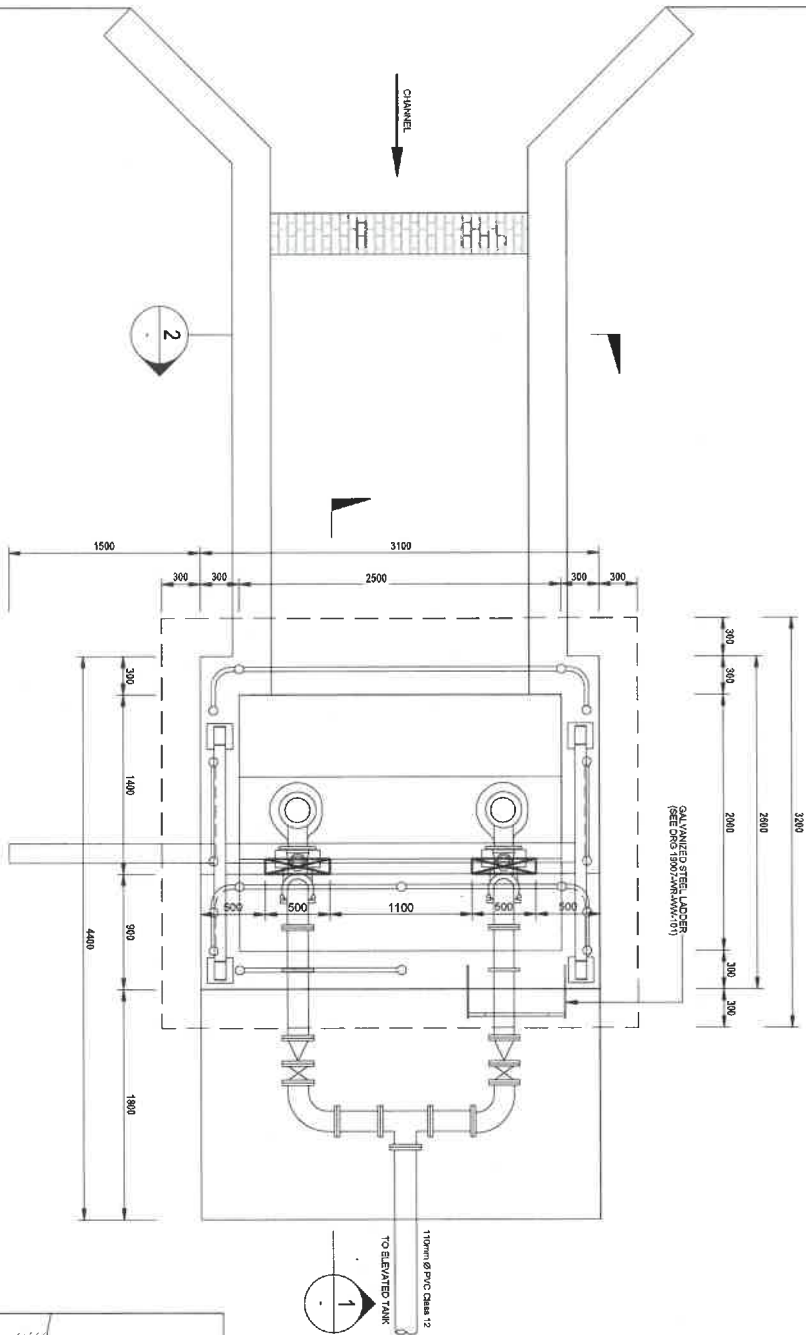
PUMP STATION PLAN SCALE 1:25
