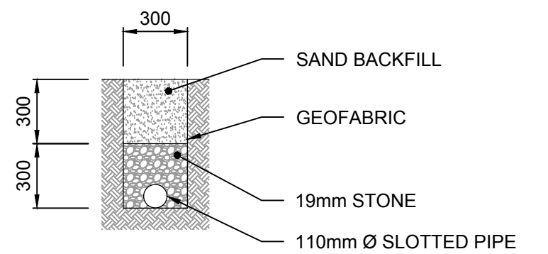
SUBSOIL DRAIN SCALE 1:25
