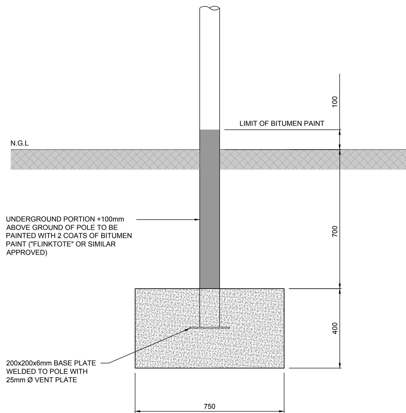
SECTION THROUGH POLE AND FOOTING SCALE 1:10
