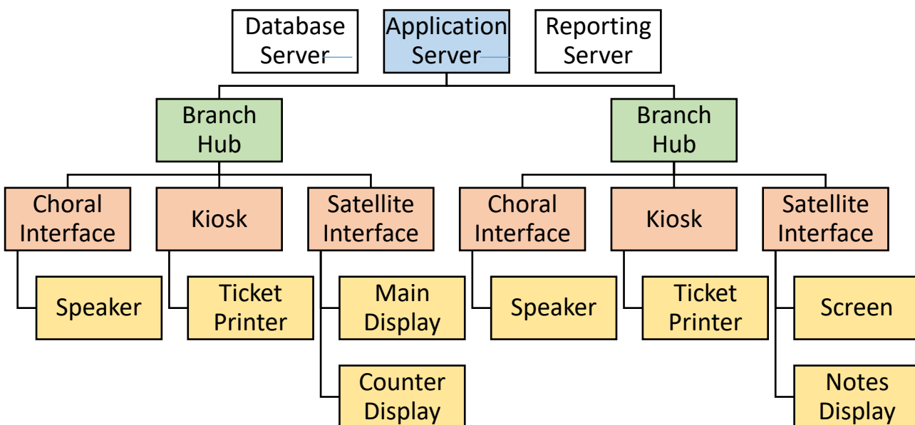
Figure 1: QMS implementation architecture
