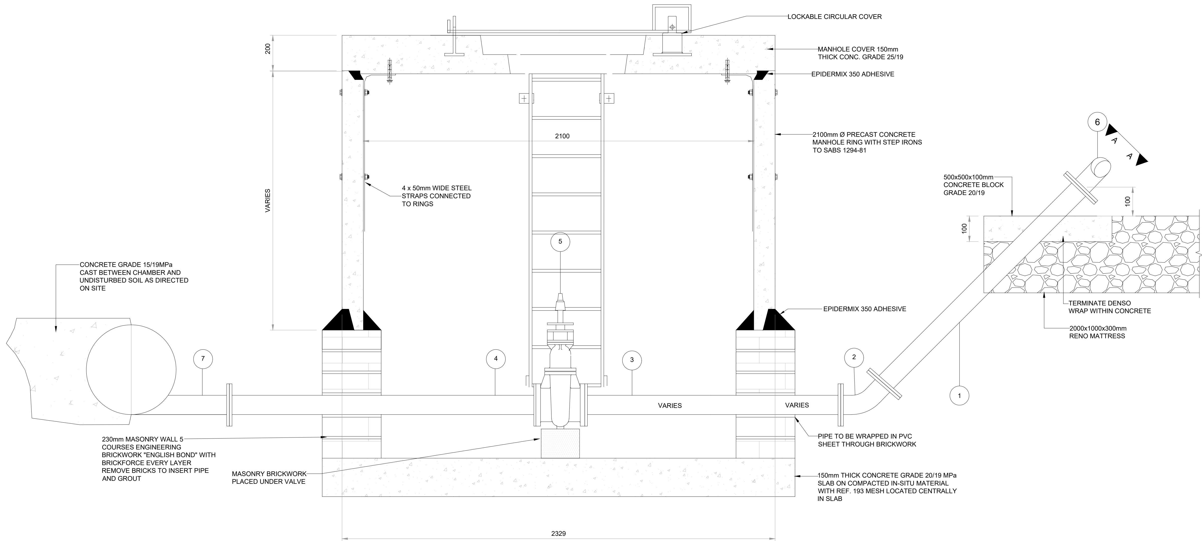
SCOUR VALVE CHAMBER SECTION SCALE 1:10
