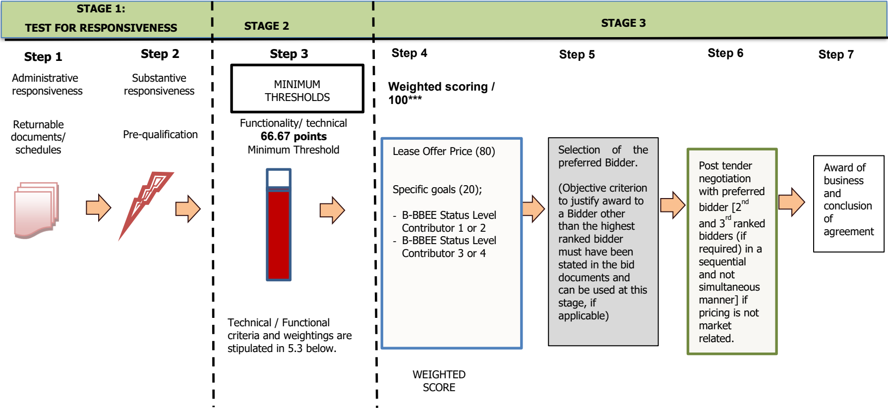
Diagram 1 Evaluation Methodology
