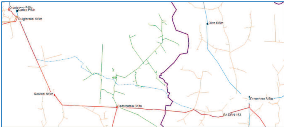
Figure 1: 132kV Network diagram
