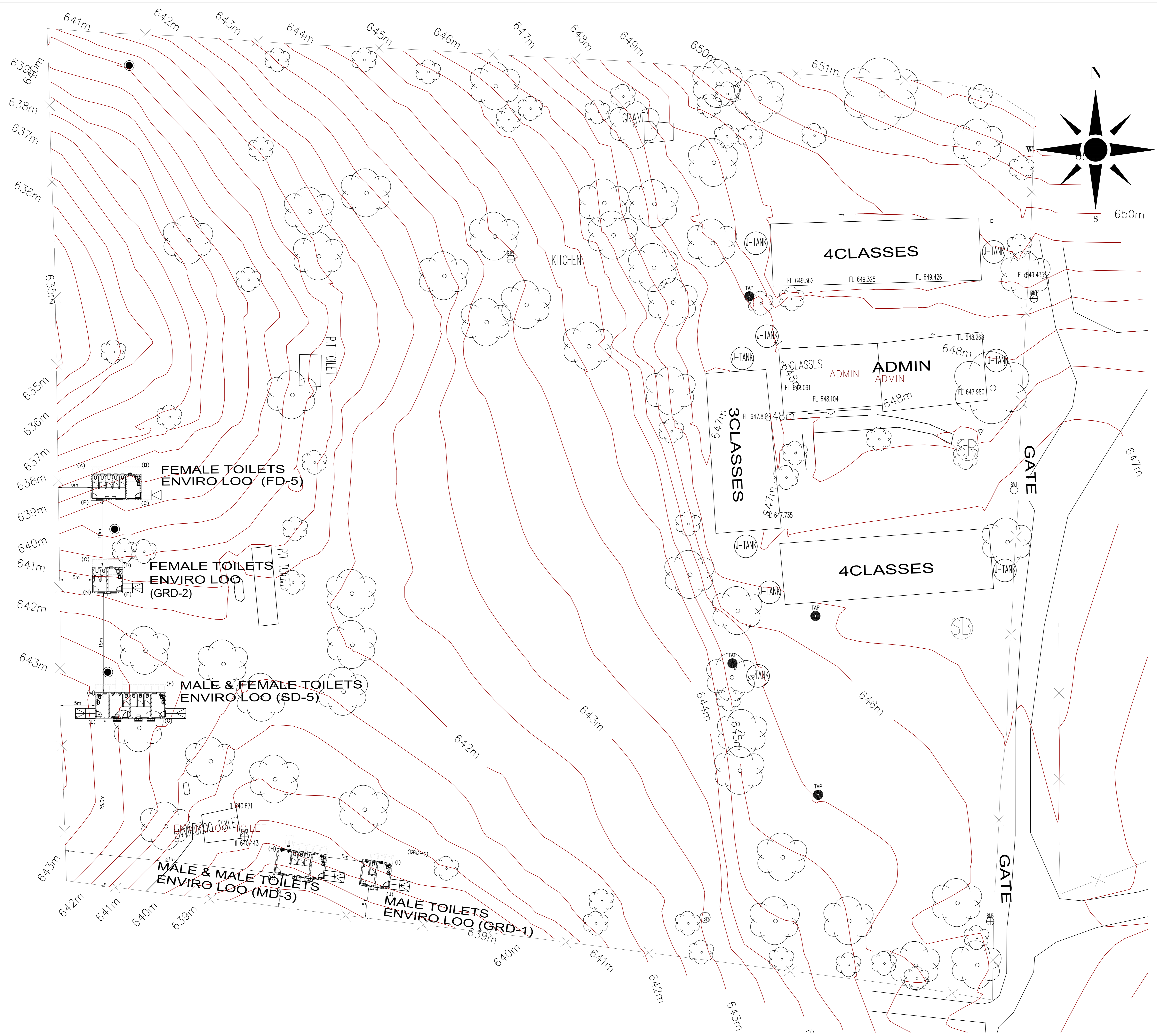
SITE DEVELOPMENT PLAN-LAYOUT (SDP)
