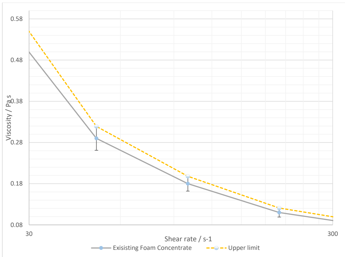
Figure 1: The viscosity versus shear rate of The Employers Existing Foam Concentrate
