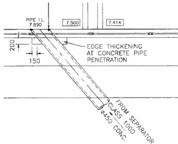
Figure 4 : Discharge pipe from manifold separator.
