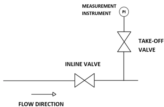
Figure 1: The figure above displays the placement of an inline and take-off valve.
