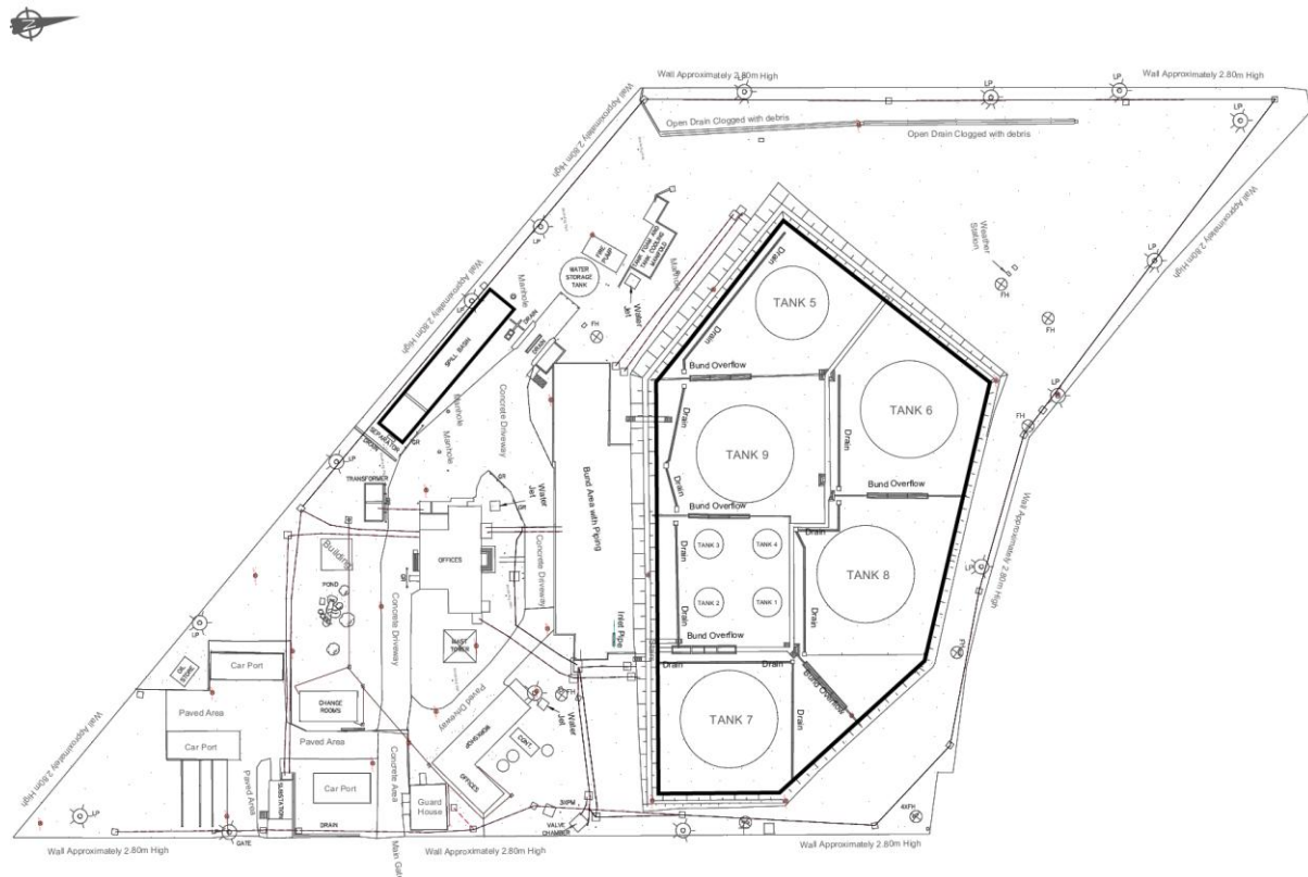
Figure 1: Measured Spill Containment areas at the Witbank depot.
