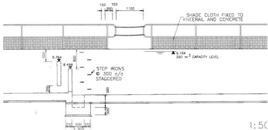
Figure 3: Capacity level
