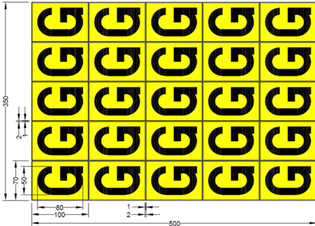
Figure 15 – Pole label "G"
