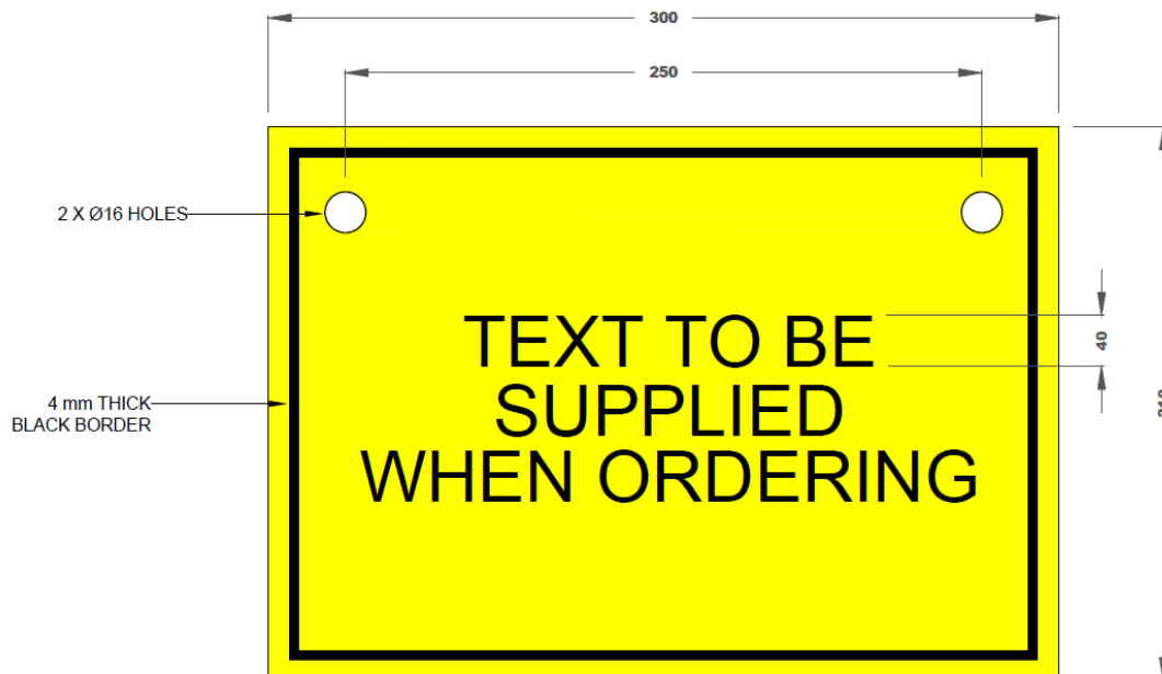
Figure 36 – Aluminium composite 132 kV line label
