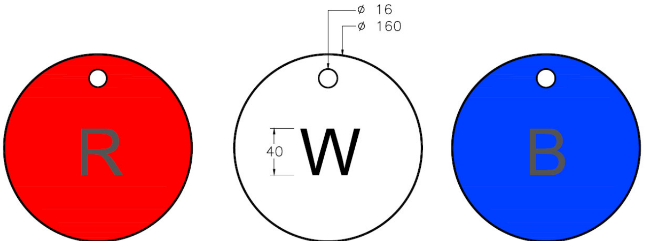
Figure 34 – Aluminium composite phase marking discs (set of 3)
