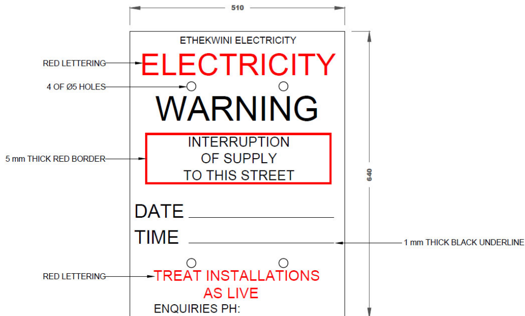
Figure 45 – Corrugated plastic warning board (English)
