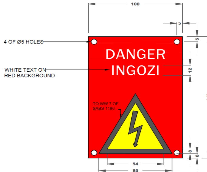
Figure 31 – Chromadek backed decal danger plate sign
