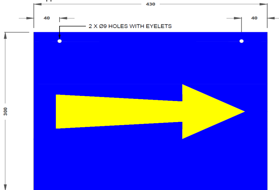
Figure 25 – Retro-reflective over laminated substation location sign
