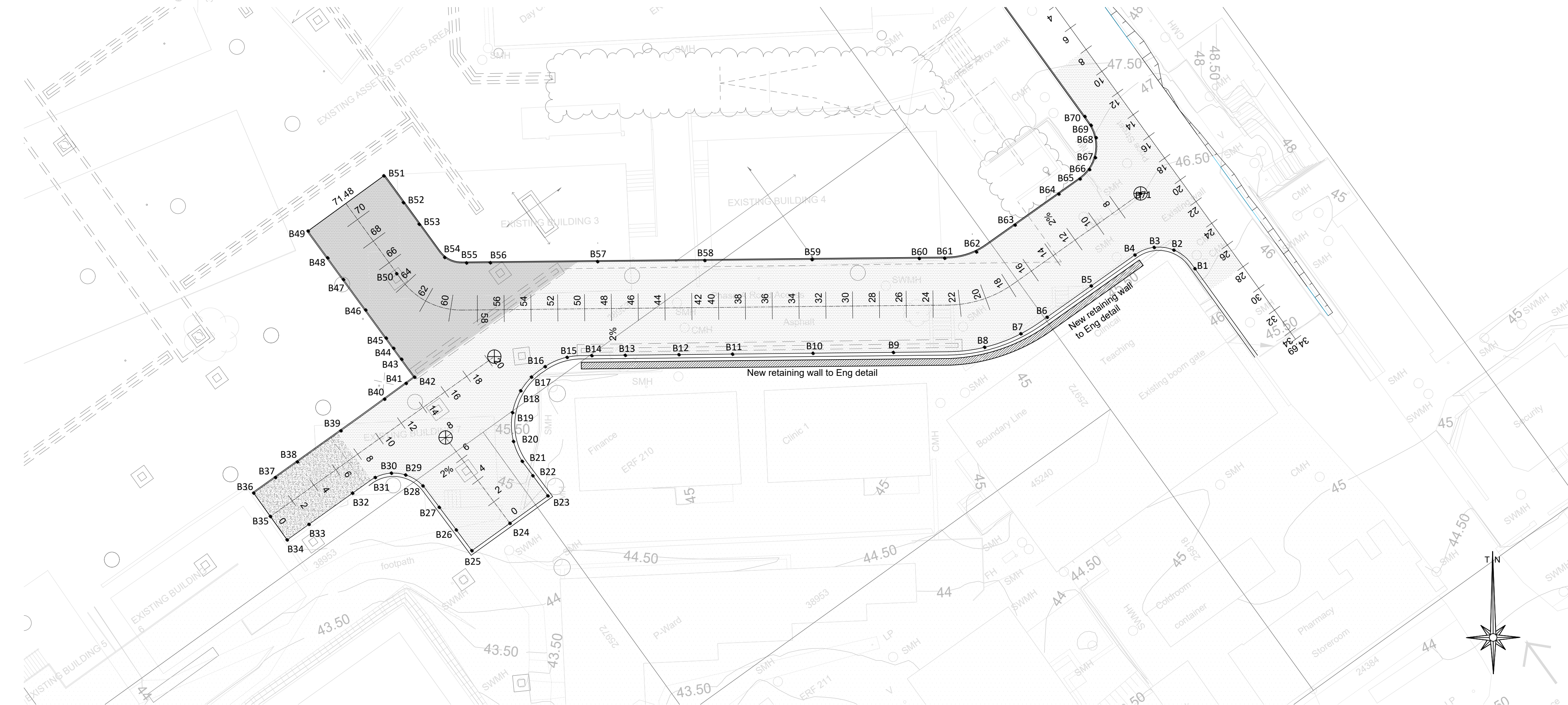
PHASE A ACCESS ROAD SETTING OUT LAYOUT SCALE 1:100
