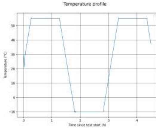
Figure 2: Environmental chamber temperature profile
