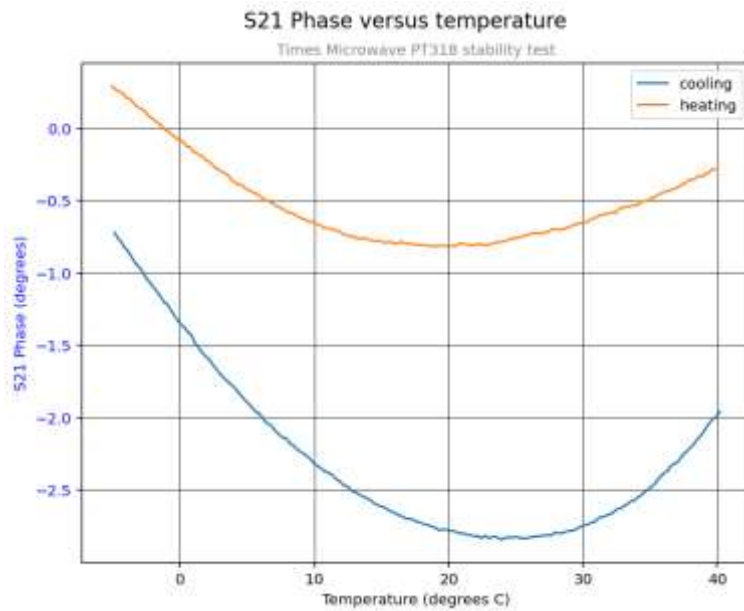
Figure 3: The phase versus temperature plot for the Times Microwave PT-318-NMSM-2.00M cable assembly
