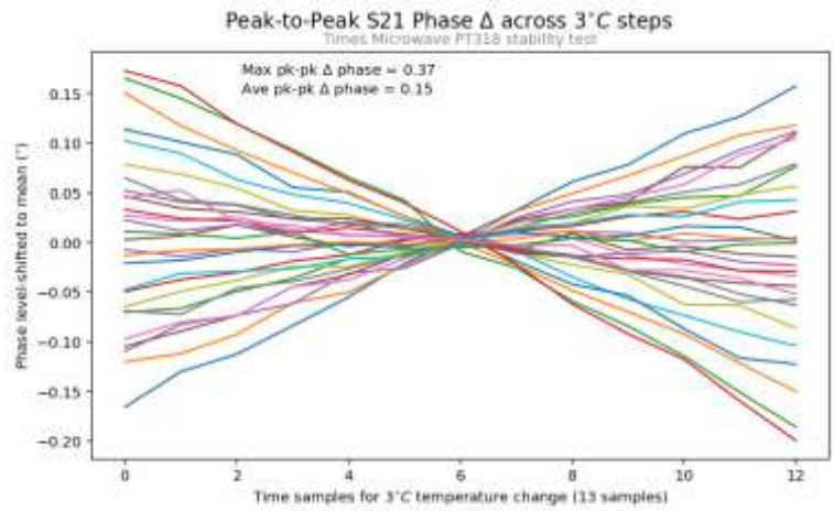
Figure 4: The combined plot showing each level shifted 3°C slice for the Times Microwave PT-318-NMSM-2.00M cable assembly
