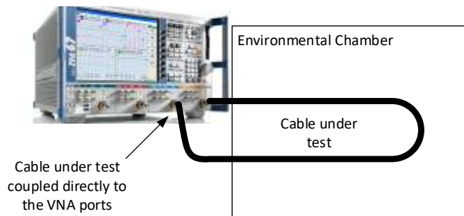
Figure 1: Insertion loss and Phase change over temperature measurement setup
