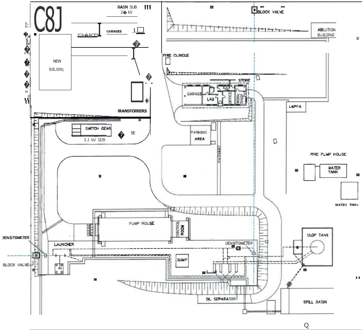
Figure 2: Bethlehem site layout
