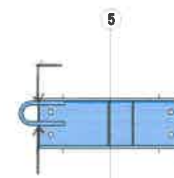
15 Bracing Bracket Type2C Front 1:10
