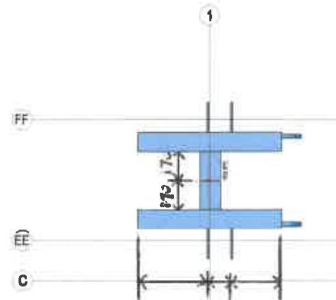
1 Bracing Bracket Type1A 1:10
