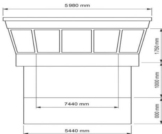
CONTROL TOWER – FRONT ELEVATION (ONE SIDE)
