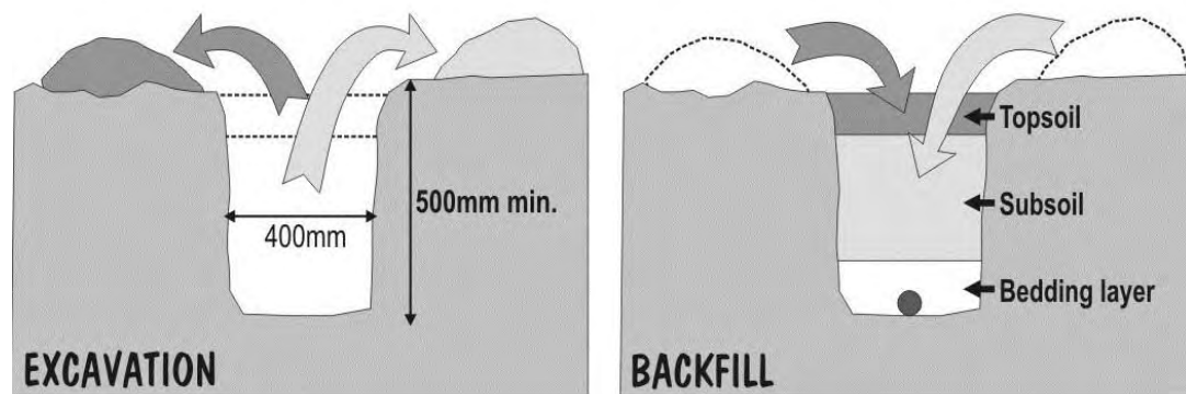
Section through a typical trenching operation
