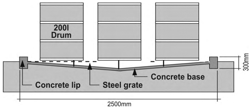
Section through a typical concrete bund
