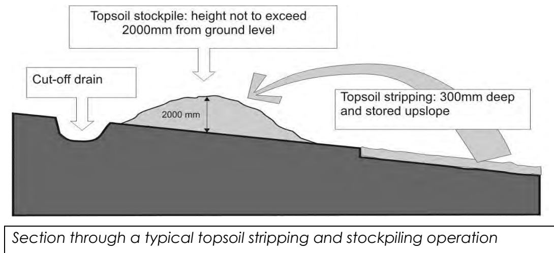
Figure 9. Section through a typical topsoil stripping and stockpiling operation
