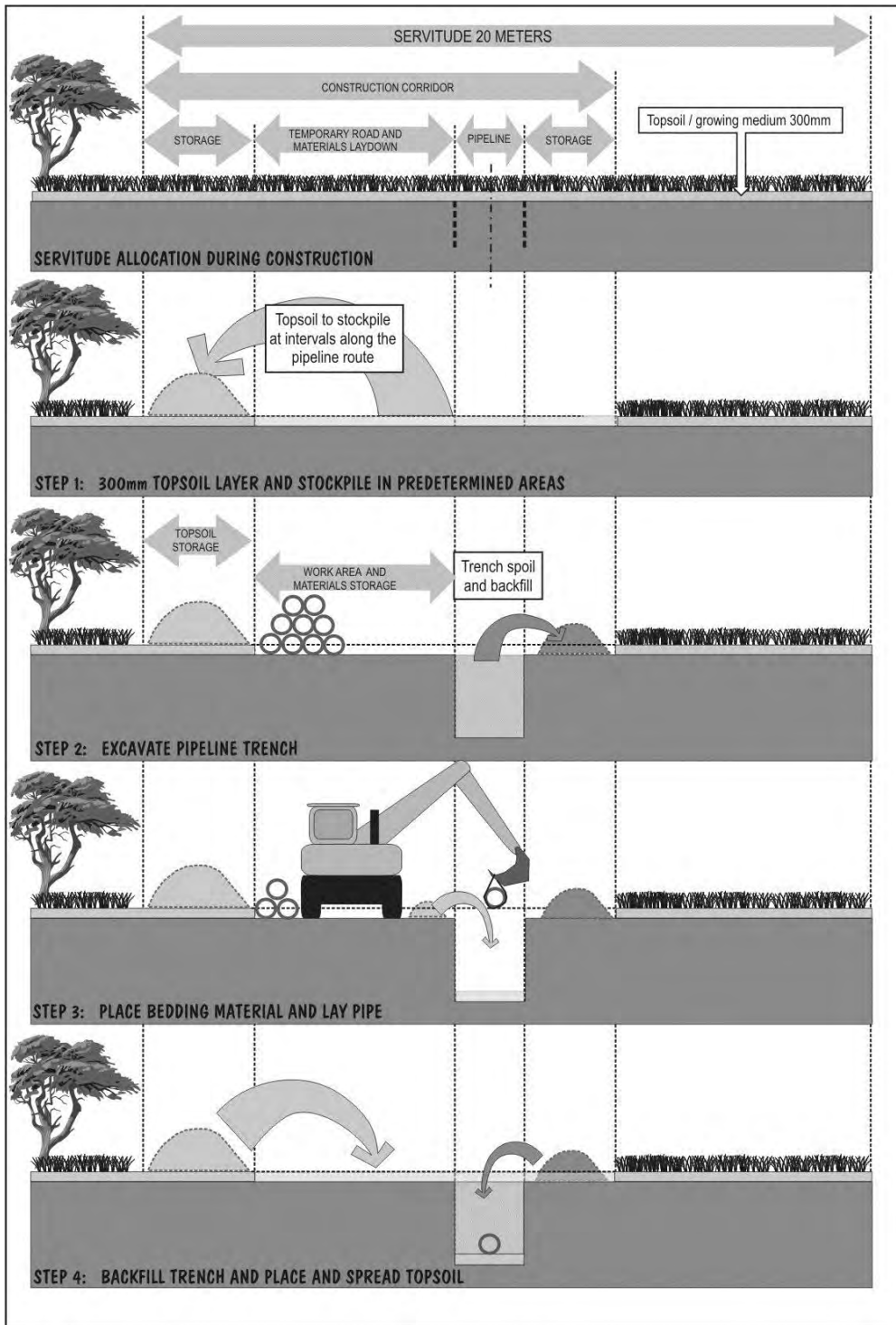
Figure 4. Works program
