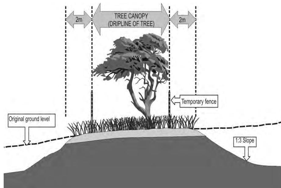
Figure 7. Section for rescue and removal of flora (Diagram as per DWA)
