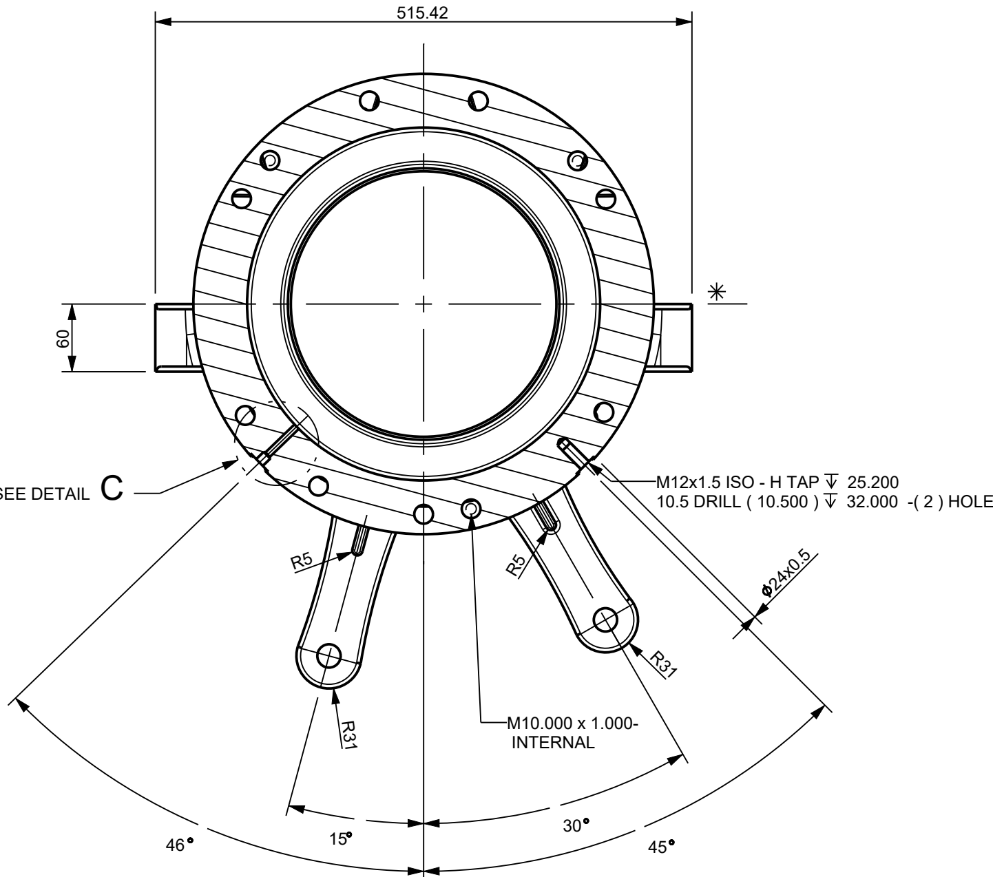
SECTION K-K
