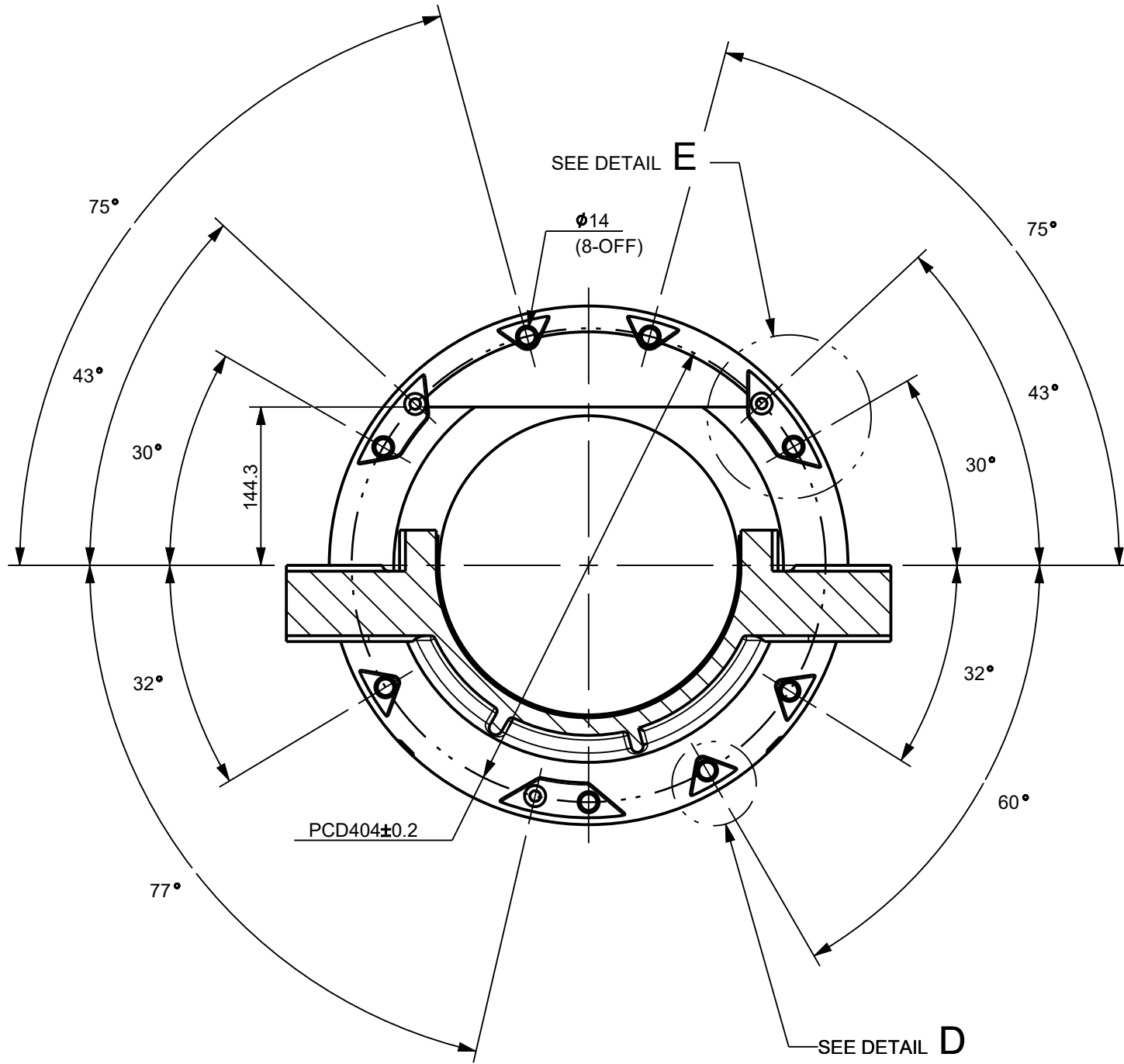
SECTION C-C
