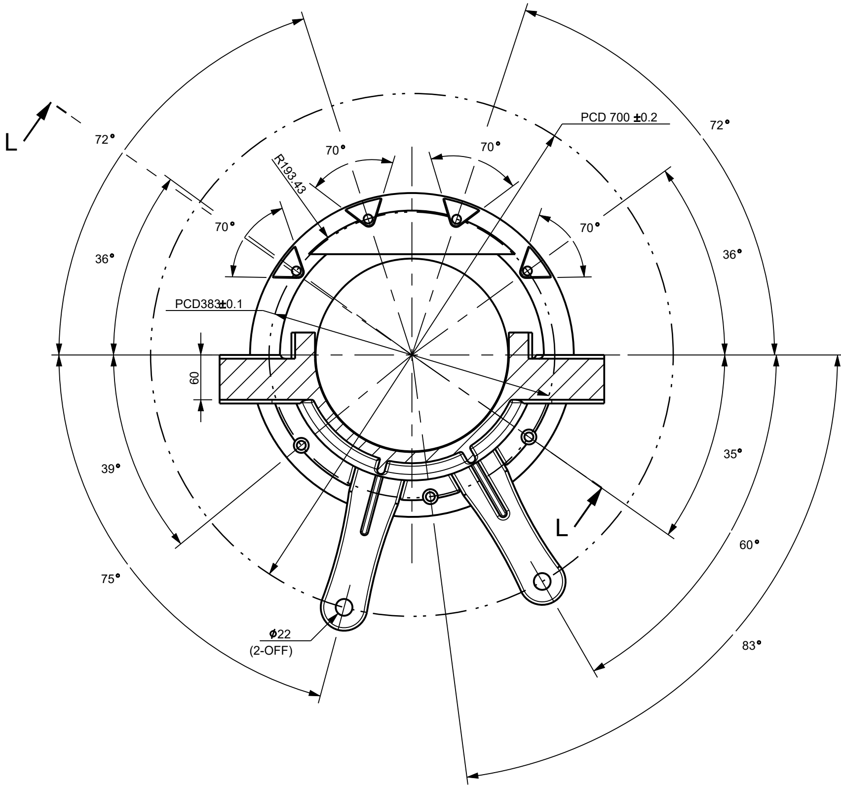
SECTION B-B
