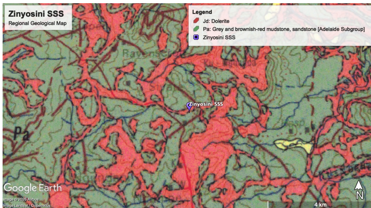
Figure 5-1: Regional geology of the site.
