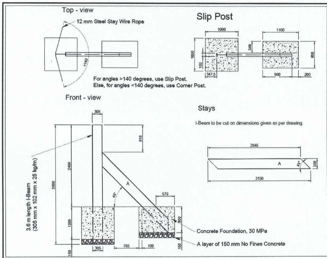
Figure 2: Slip posts
