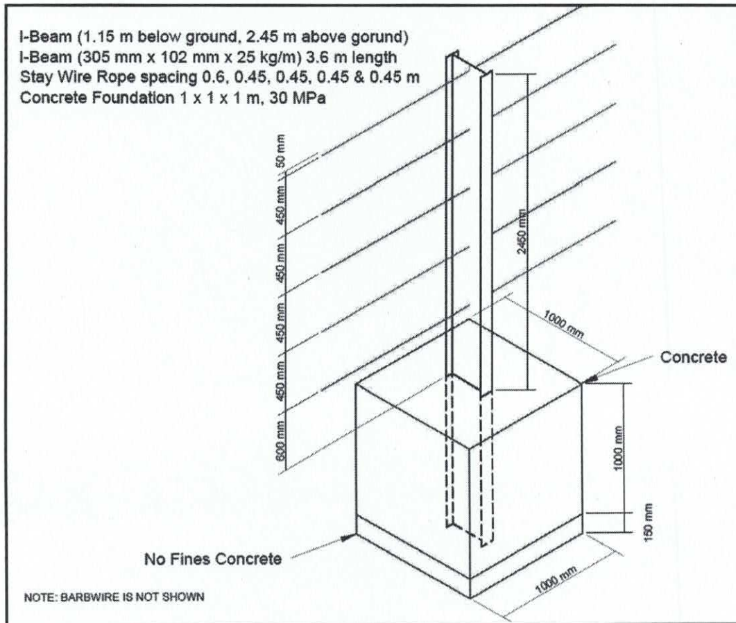
Figure 4: Line posts
