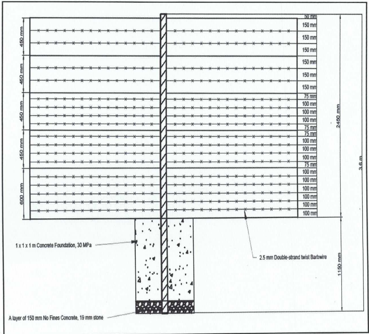
Figure 6: Strand configuration for River front fence
