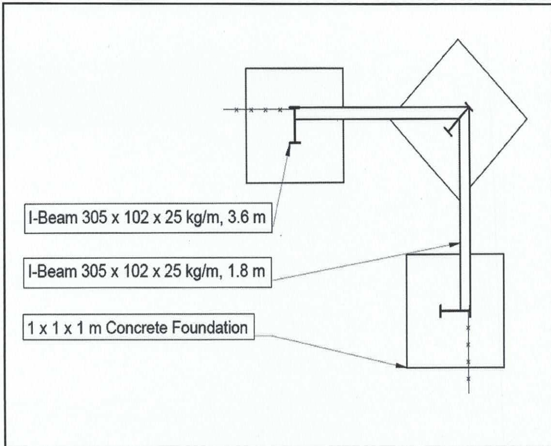
Figure 1: Corner posts
