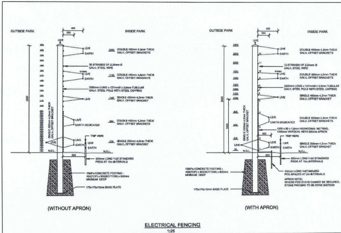
Figure 7: Electrical Fencing
