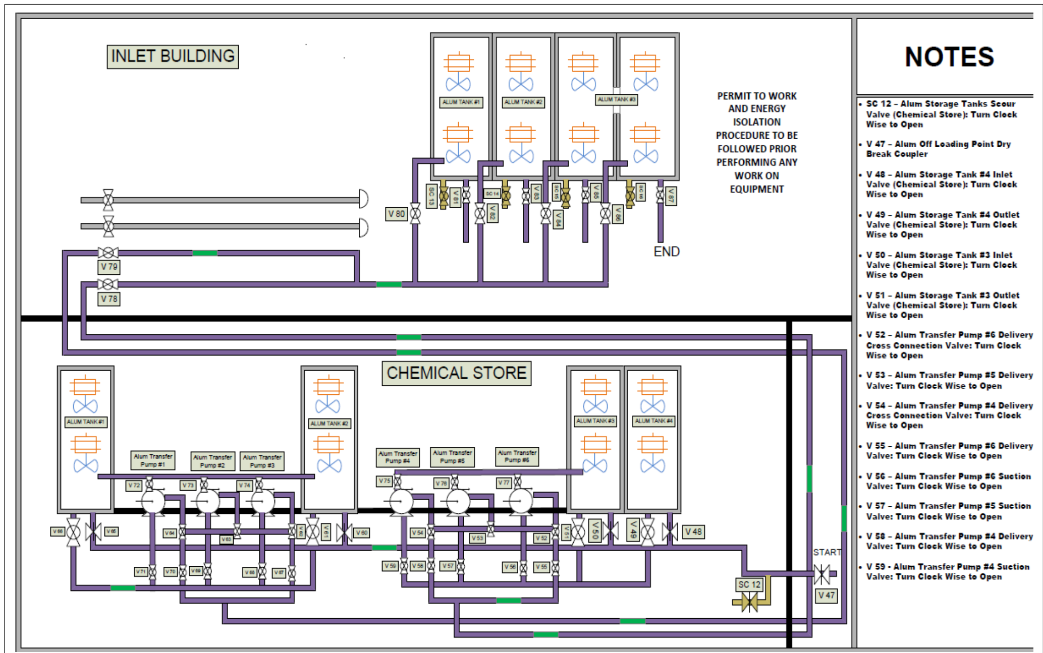
DIAGRAM 1 – A GENERAL LAYOUT OF A ALUMINIUM SULPHATE STATION
