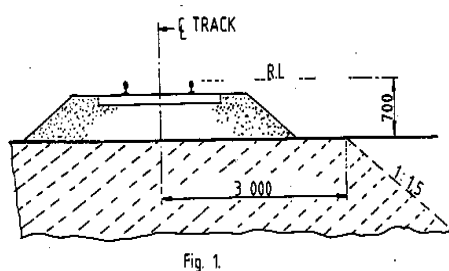
Formation level
