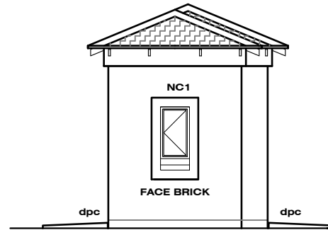
SIDE ELEVATION 1:100
