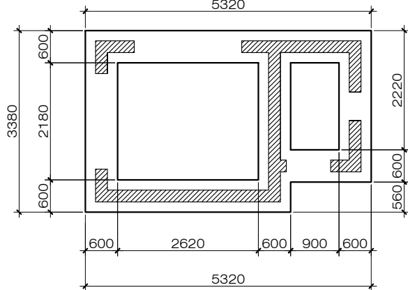
FOUNDATION PLAN 1:100
