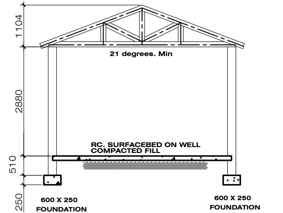
TYPICAL SECTIONAL ELEVATION 1:100
