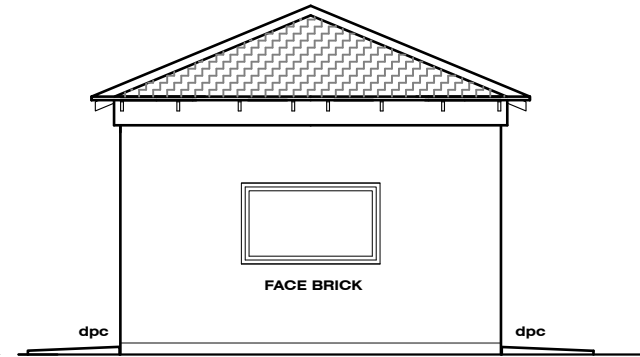
BACK ELEVATION 1:100
