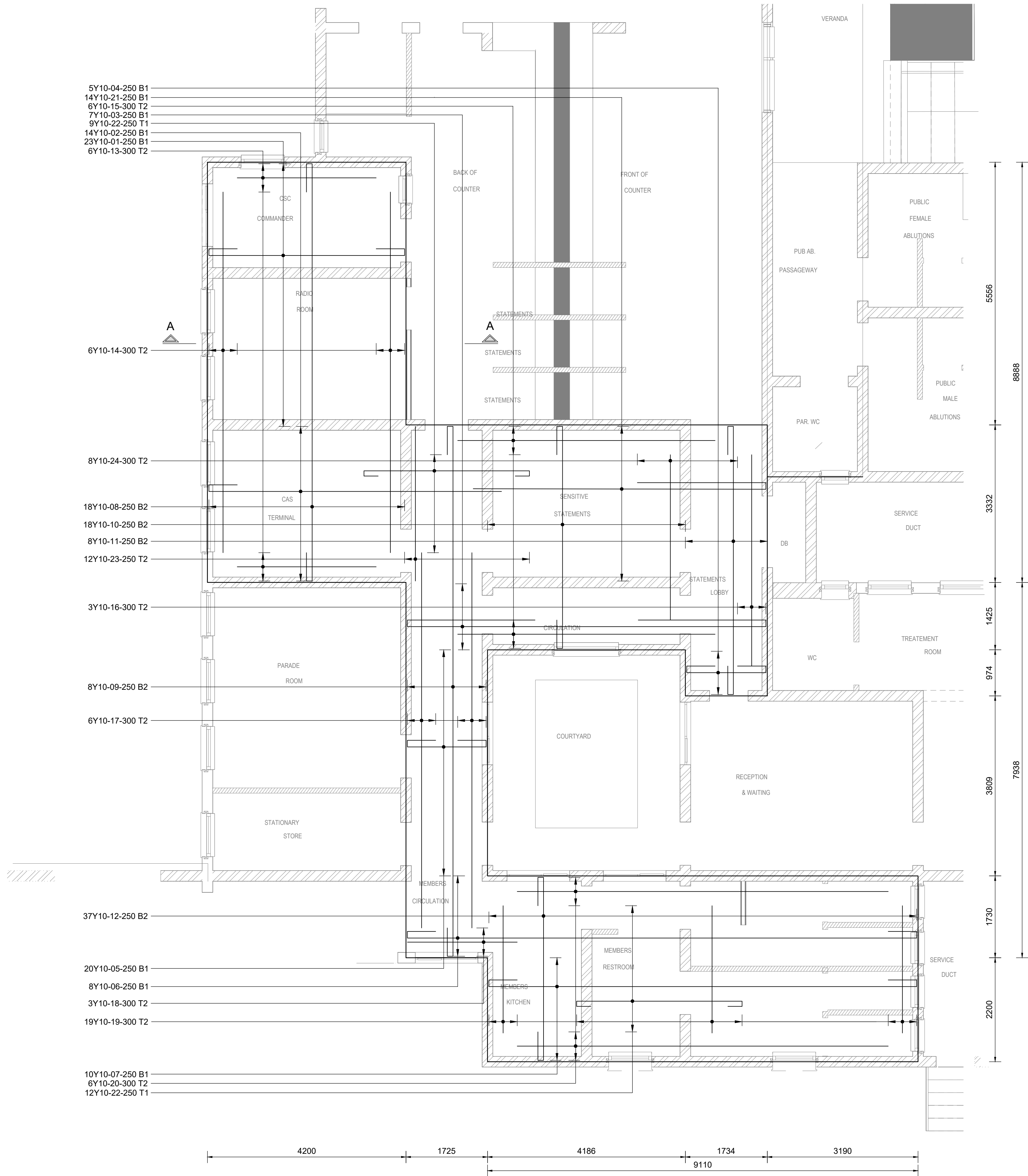
ROOF SLAB REINF. LAYOUT SCALE 1:50
