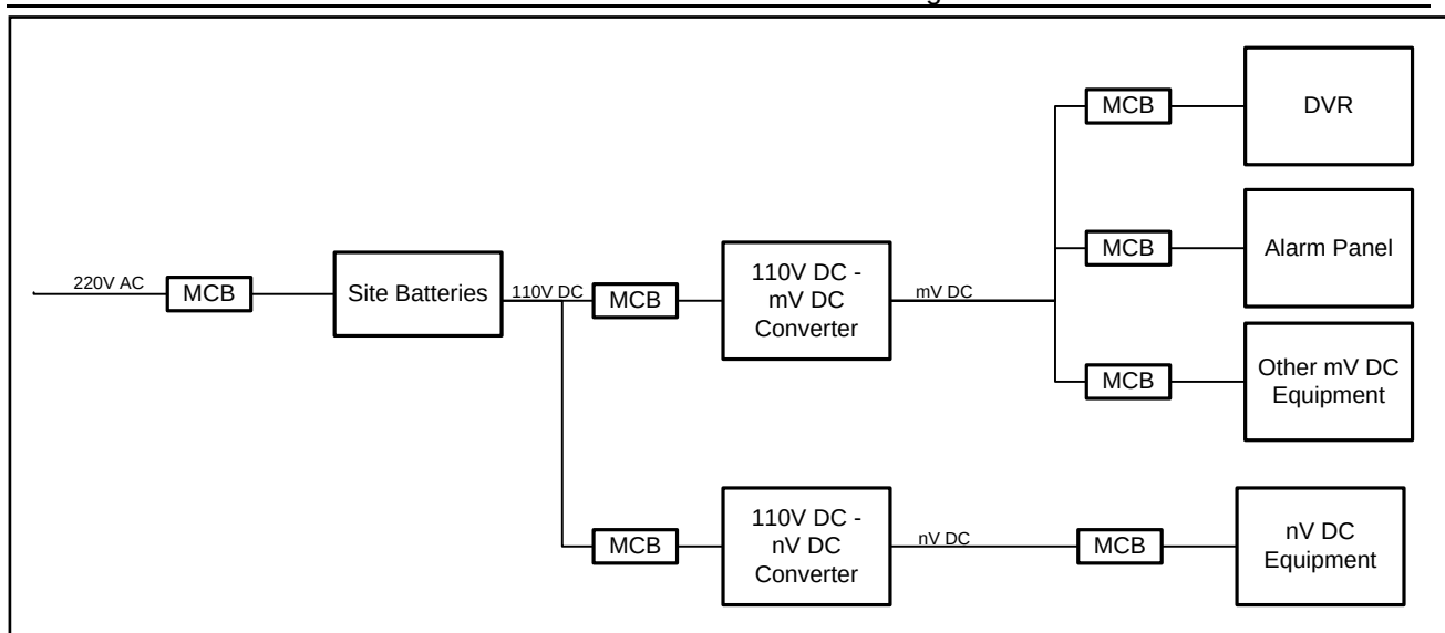
Figure 9: Preferred Power Distribution, Using Backup Power from the Site
