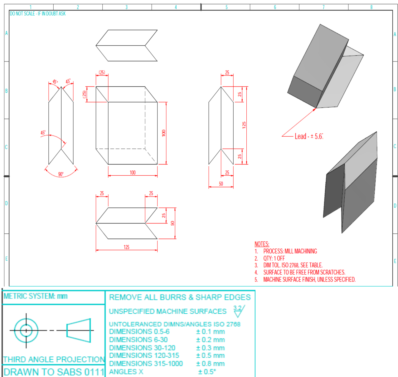
Figure 1: Lead Bricks - Drawing scale 1:2
