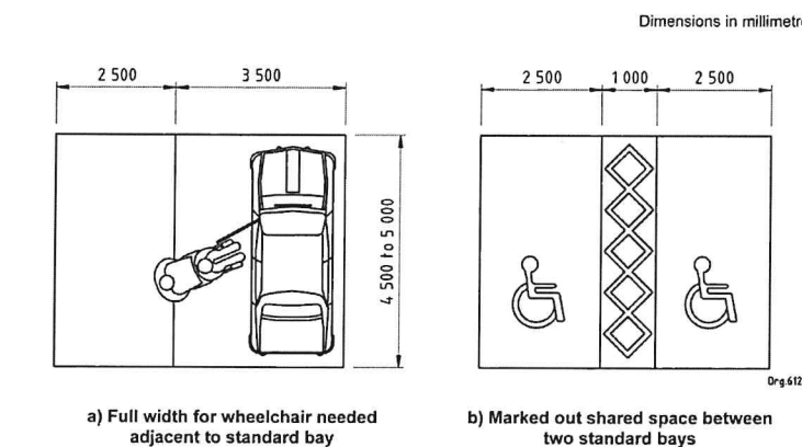
Figure 2 — Accessible parking bays
