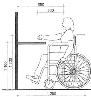
Figure 2 - Reach range over an obstacle (Muller, 2013)
