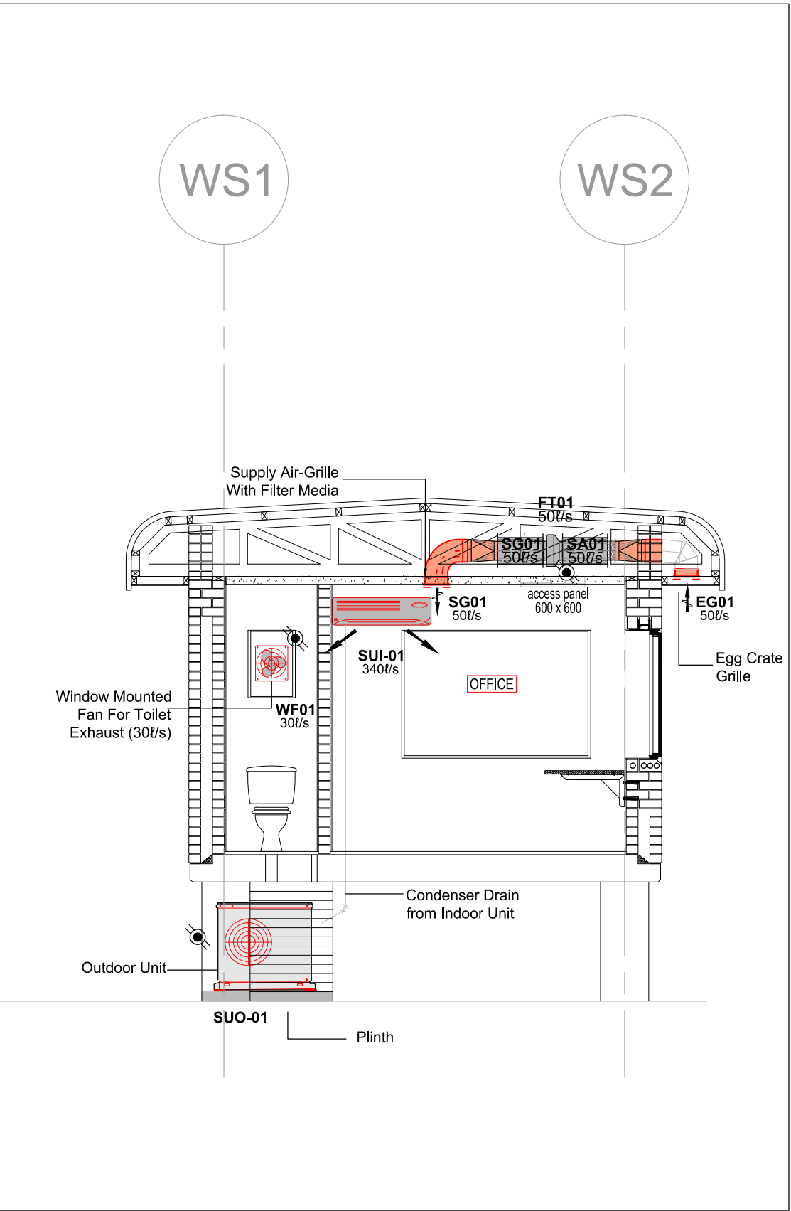
SECTION (A - A) SCALE 1:50
