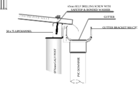
GULLY CHANNEL FIXED TO GULLY POST BRACKET BY MEANS OF 40mm x 12mm ALU R-CLIP RIVETS
