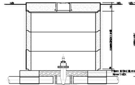
SECTION DETAIL OF VALVE BOX
