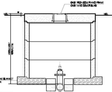
SECTION DETAIL OF VALVE BOX
