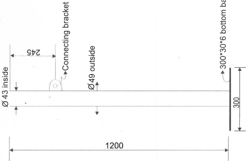
Drawing 11: Rain Gauge Stand
