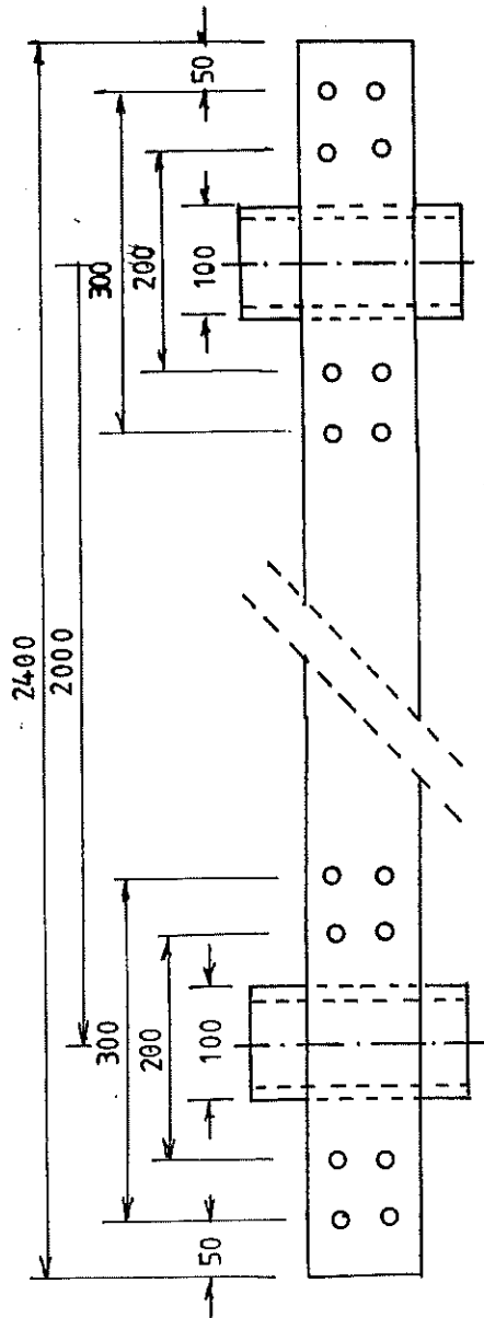
PLAN VIEW SCALE 1:75
