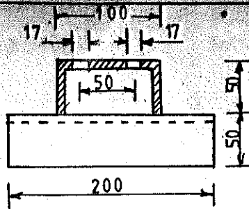
FRONT VIEW SCALE 1:5 (CHANNEL IRON)
