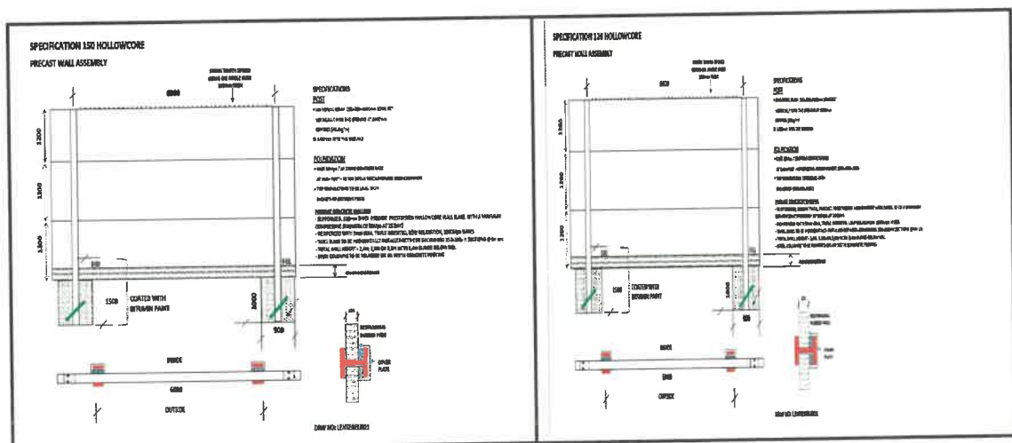
Specification drawings for the Fence/Wall
