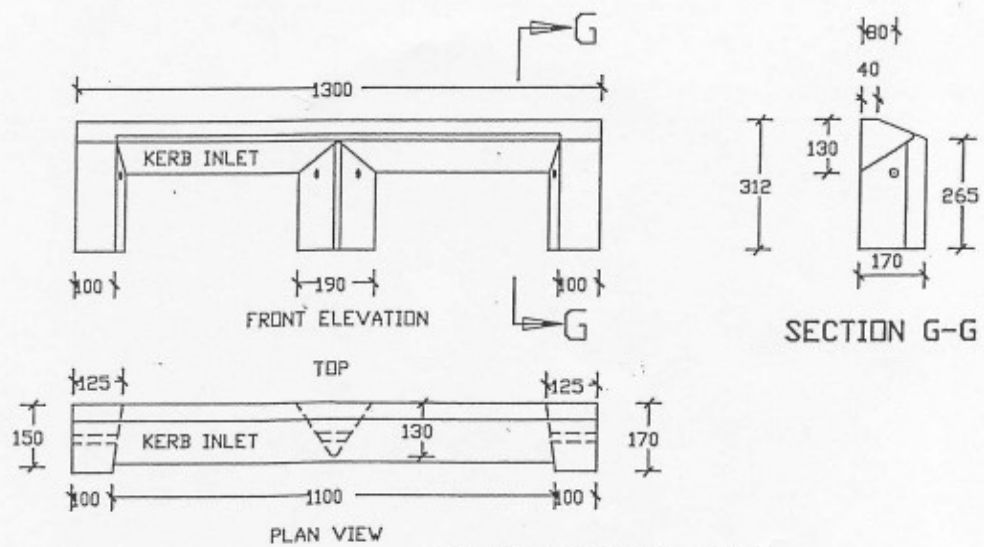
DETAILS OF PRE-CAST KERB INLET TO SUITE CK5 (PAROW TYPE) KERB
