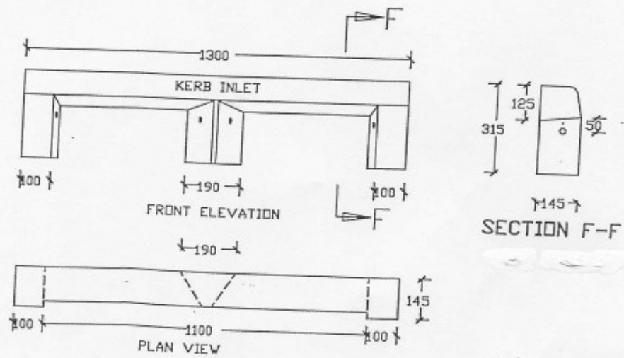
DETAILS OF PRE-CAST BARRIER KERB INLET
