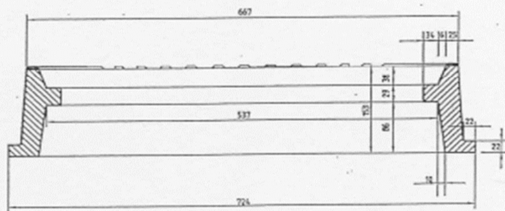
SECTION A -A THROUGH FRAME
