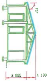
SECTION 01-01 SCALE 1:100
