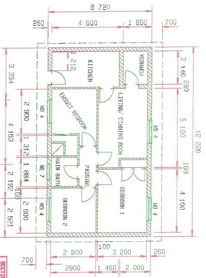
NEW FLOOR PLAN LAYOUT SCALE 1:50
