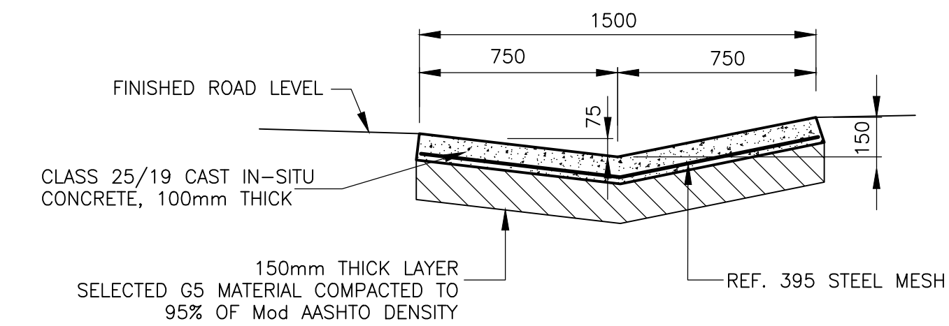
TYPE 1: SMALL SIDE DRAIN ALLOWING ERF ACCESS
