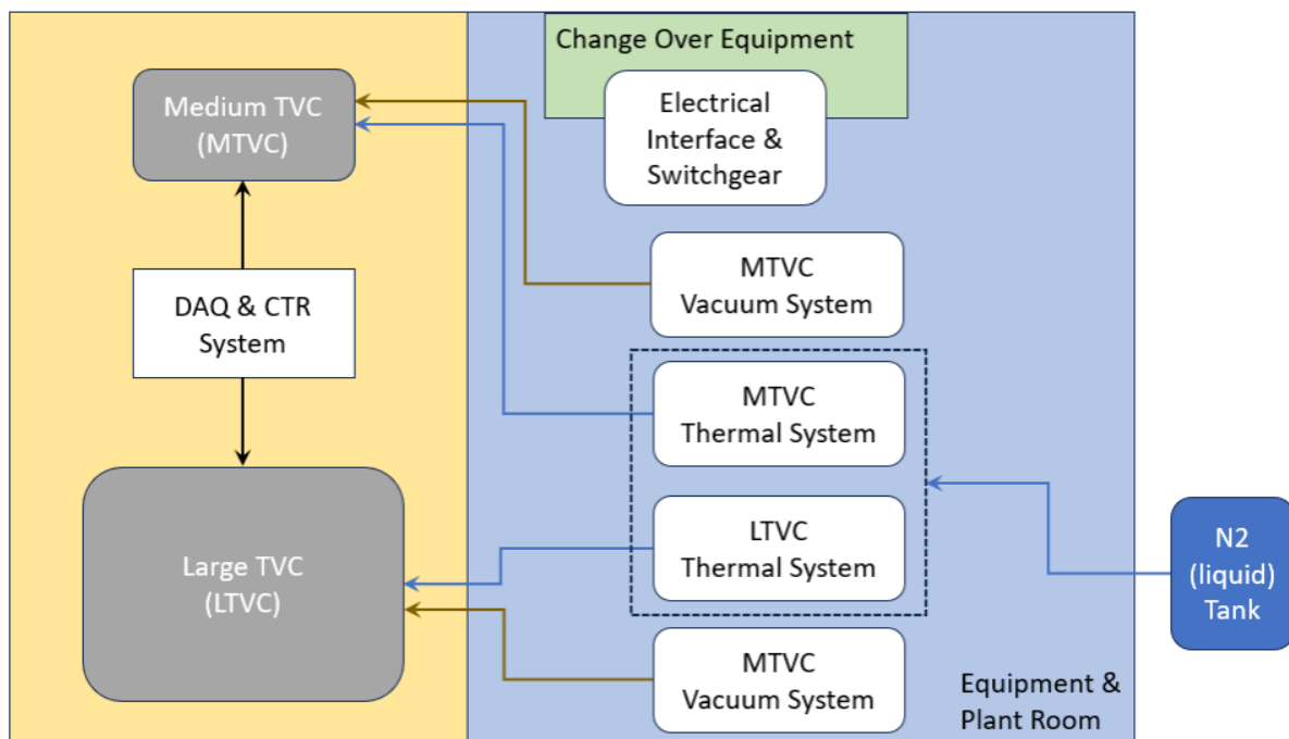
Figure 2. Thermal Vacuum TVC System Overview Schematic
