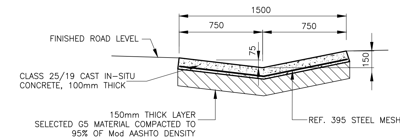
TYPE 1: SMALL SIDE DRAIN ALLOWING ERF ACCESS
