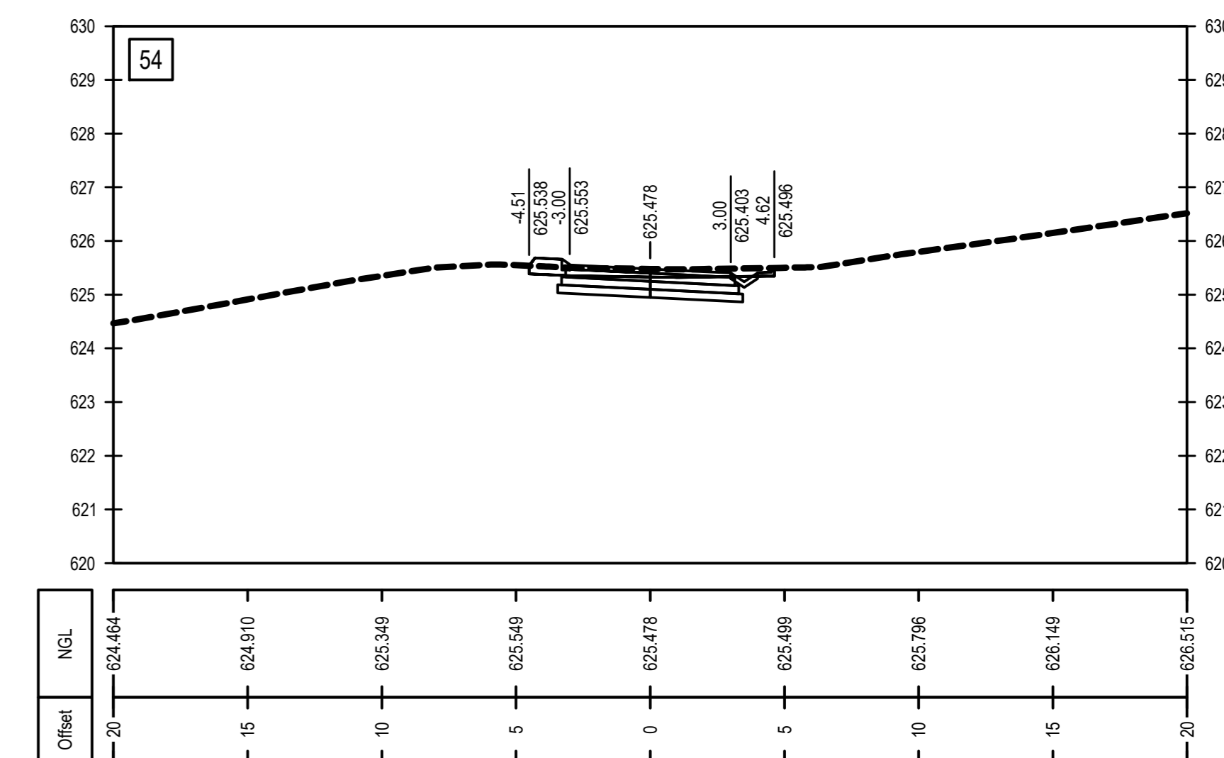
CROSS SECTIONS INTERSECTION 5 FROM 0.00 TO 54.00
