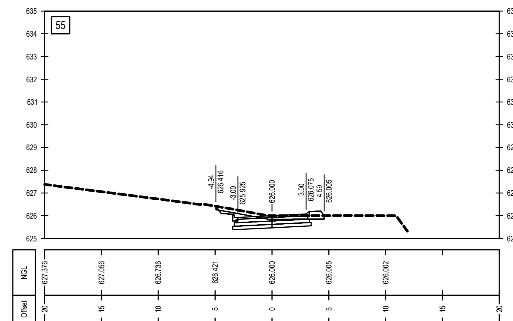
CROSS SECTIONS INTERSECTION 4 FROM 0.00 TO 55.00
