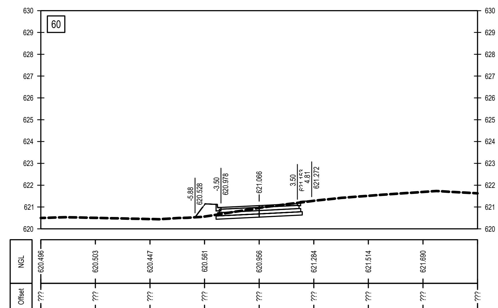
CROSS SECTIONS INTERSECTION 3 FROM 0.00 TO 69.00
