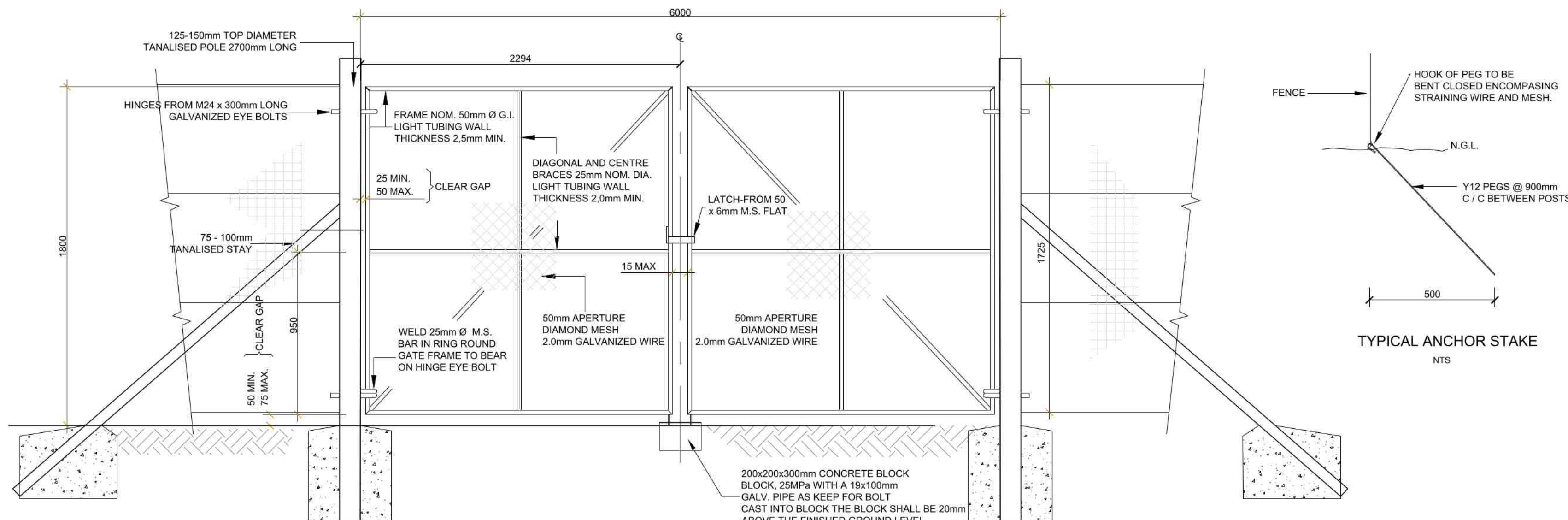
NOTE: 1. GATES ARE SYMMETRICAL ABOUT CENTRE LINE & FITTED WITH LOCKING DEVICE
