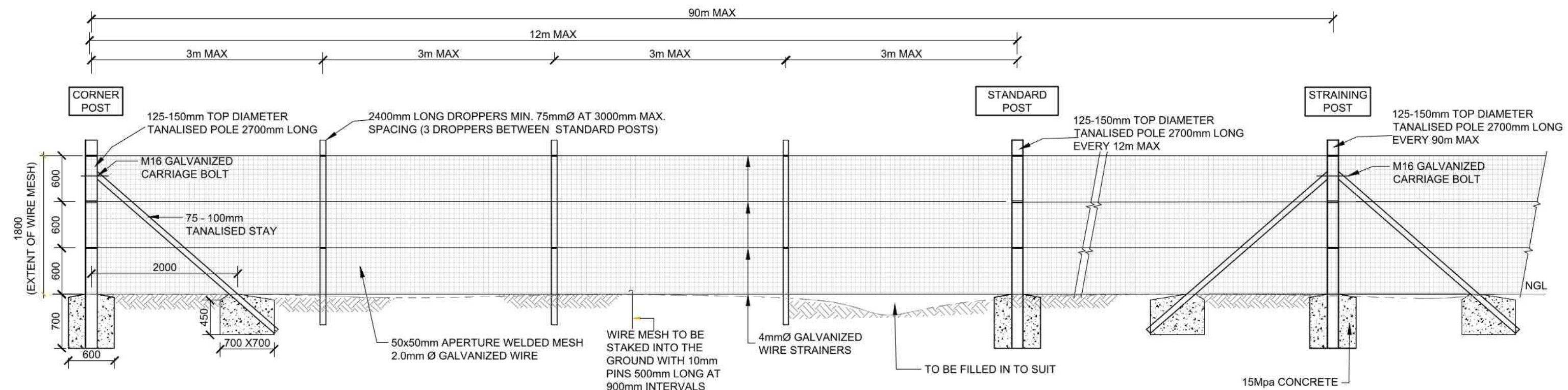
GENERAL DETAILS OF 1.8m HIGH SECURITY FENCE FOR GRADE R SCALE 1:50
