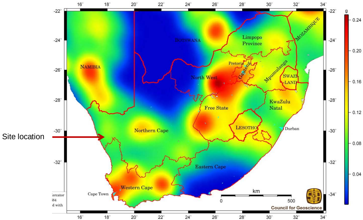
Figure 4: Peak ground acceleration (g) with 10% probability for being exceeded in a 50 year old period.
