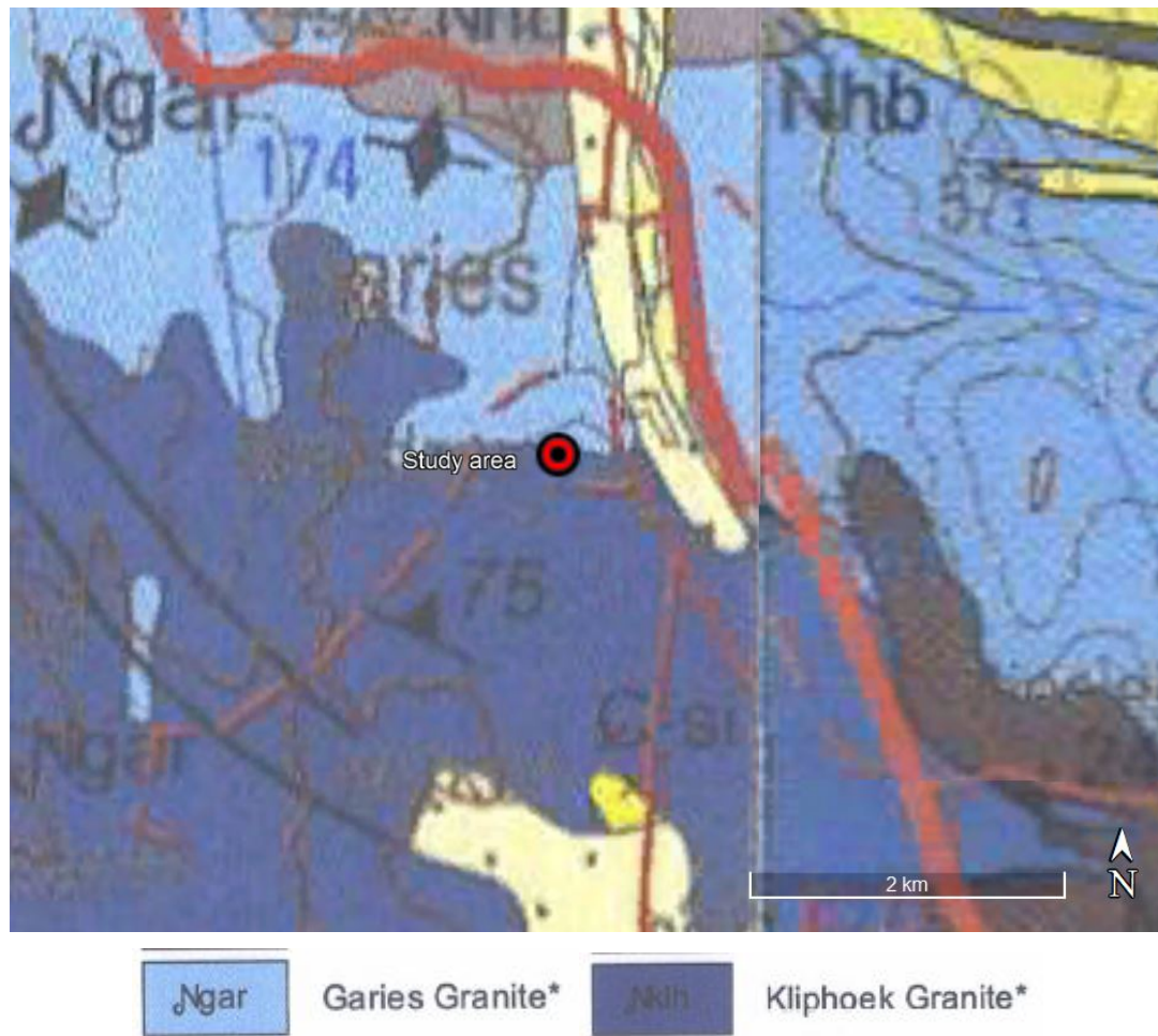
Figure 5: Showing the general geology map of the site area ( red dot ); (Geological Survey, printed by the Government Printer, Republic of South Africa 2011).
