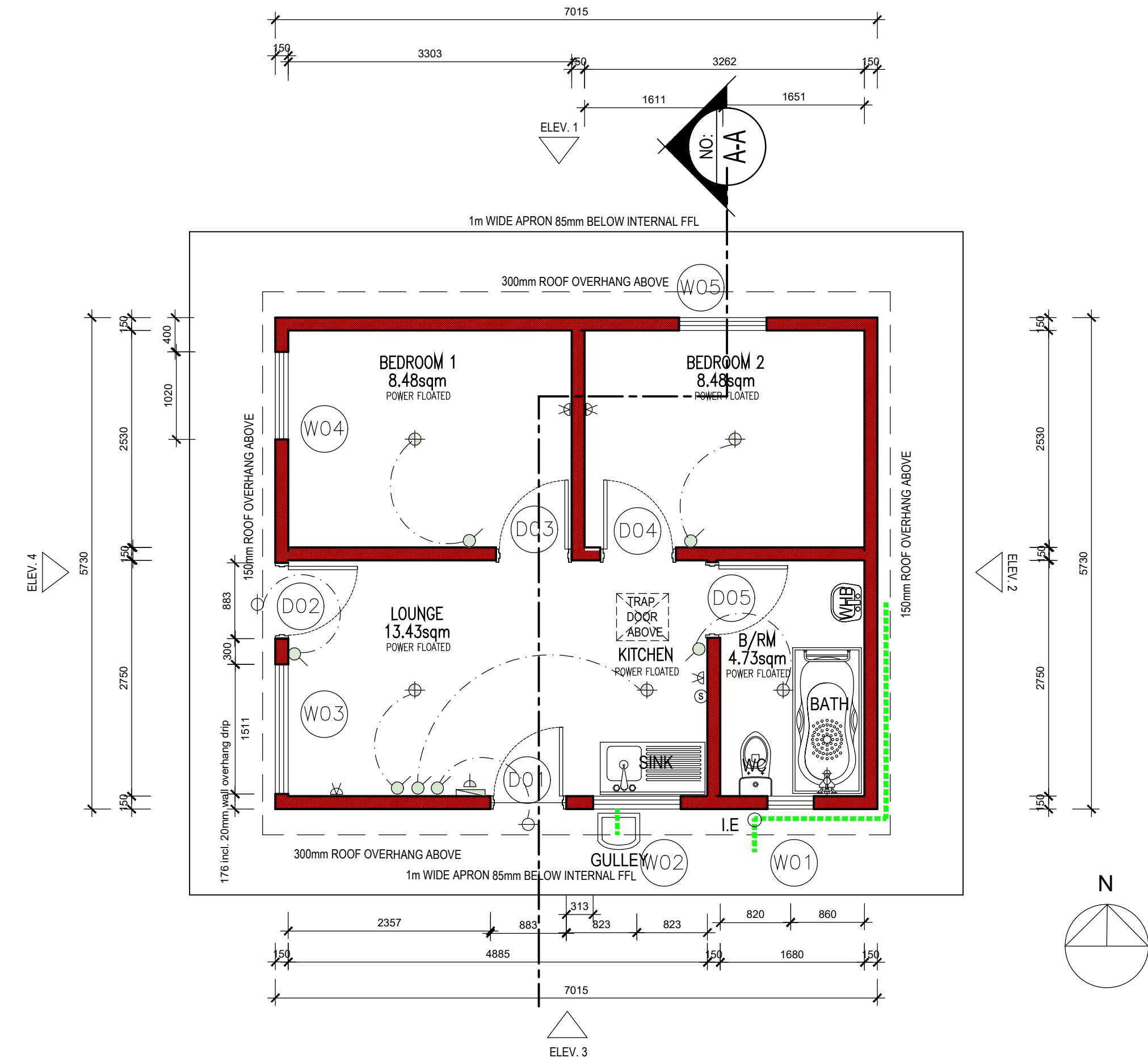
PLAN - 1/50
