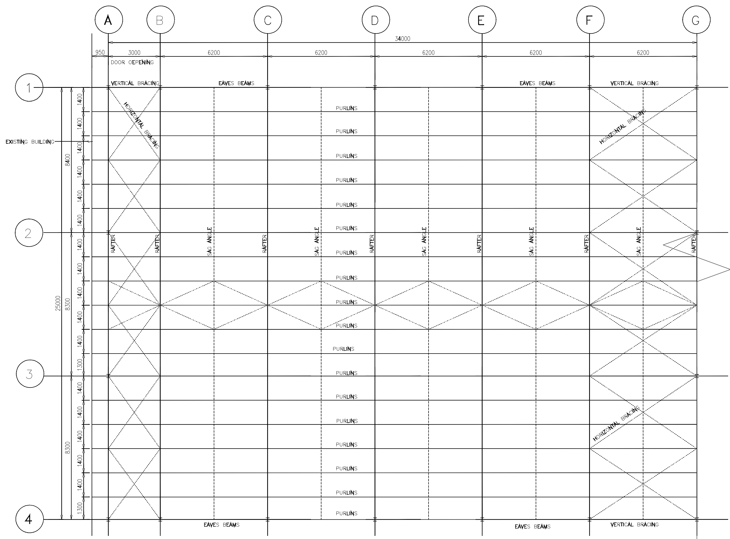
ROOF LAYOUT SCALE 1:100
