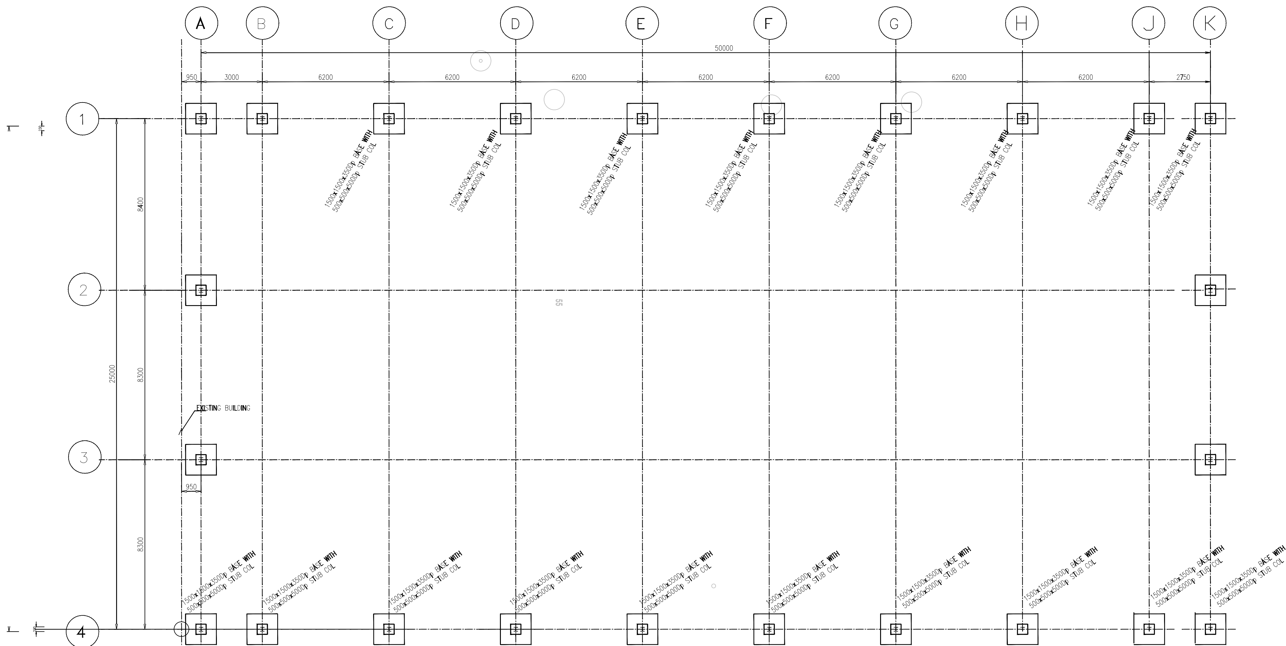
FOUNDATION LAYOUT SCALE 1:100
