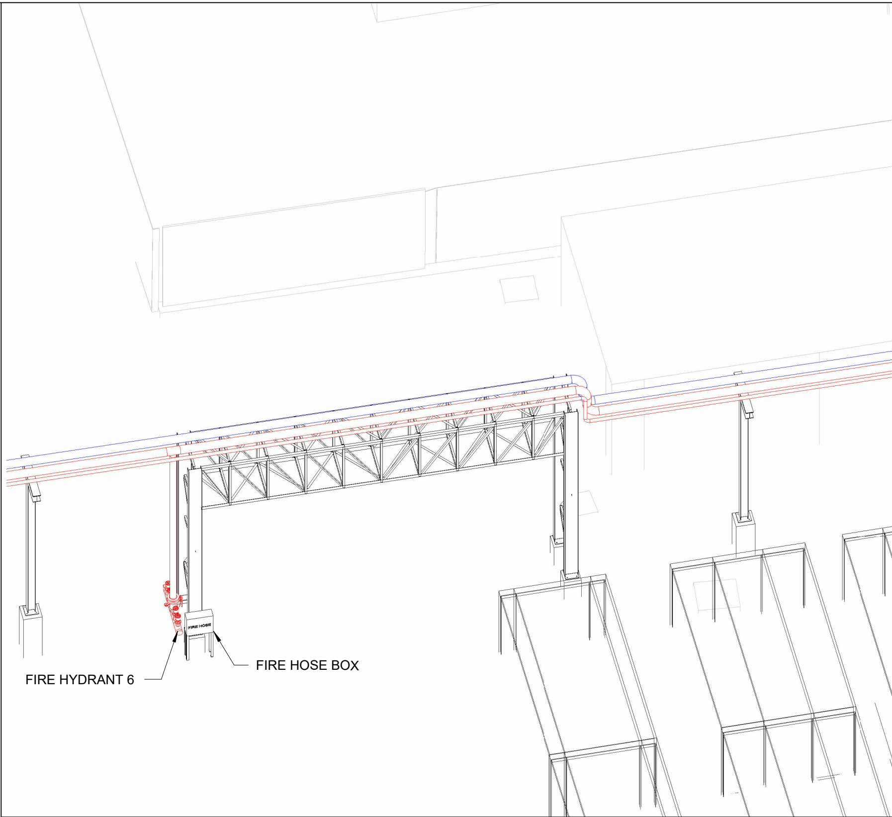
3D VIEW OF PIPE BRIDGE 2
