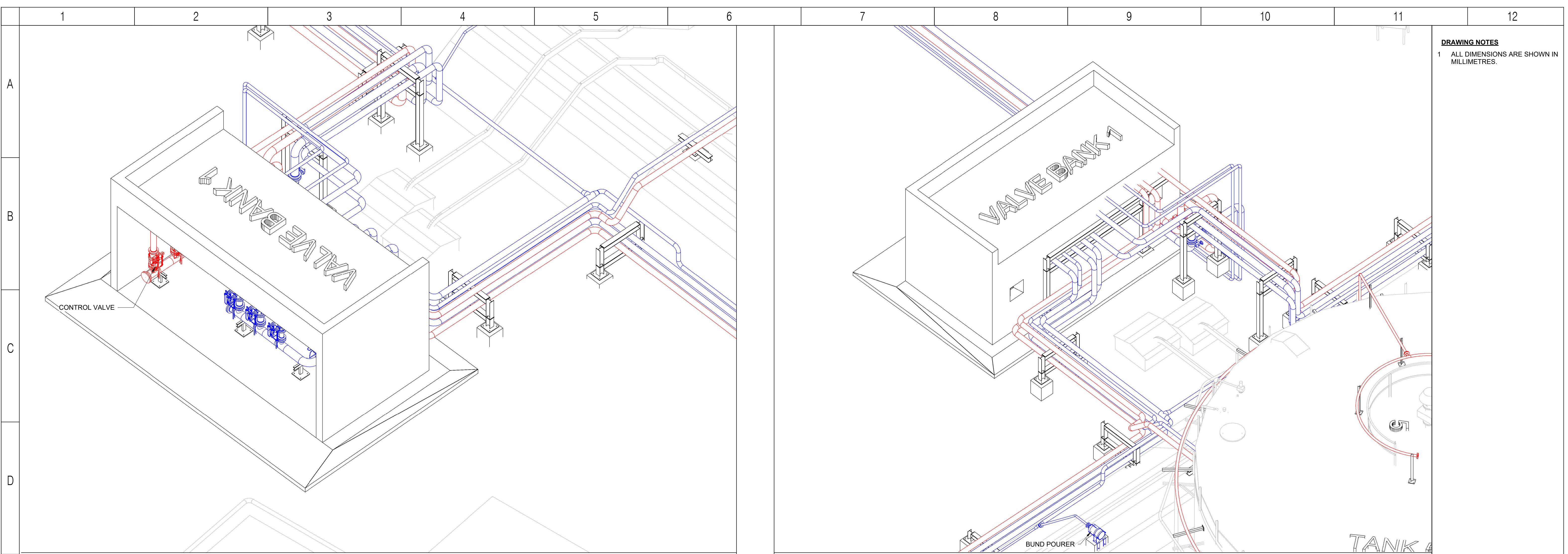
3D VIEW OF FRONT OF VALVE BANK ONE
