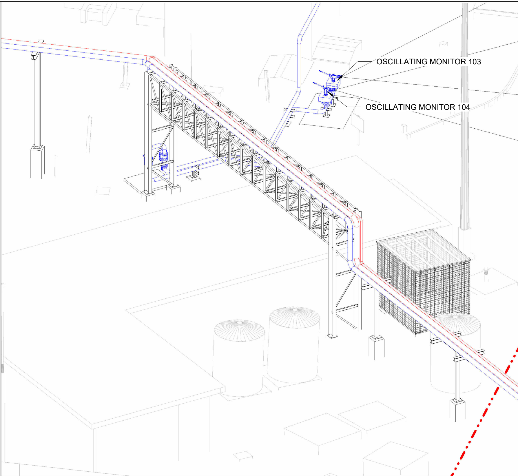
3D VIEW OF PIPE BRIDGE 3
