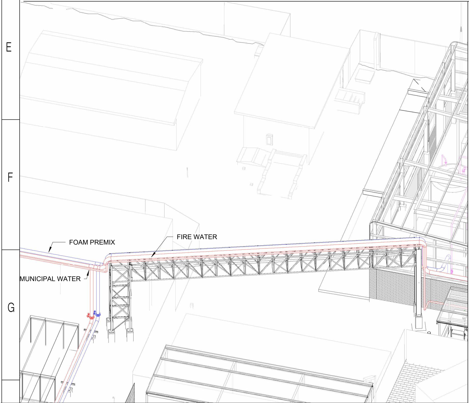
3D VIEW OF PIPE BRIDGE 1
