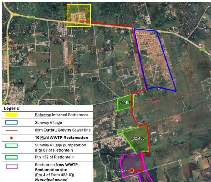
FIGURE 3: LAYOUT MAP OF THE NEW WWTP
