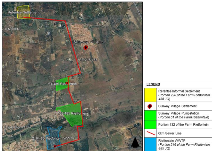
FIGURE 1: LOCALITY MAP FOR UPGRADE OF RIETFONTein WWTP
