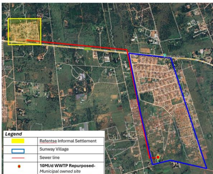
FIGURE 2: LOCALITY MAP FOR THE REHABILITATION OF THE OXIDATION PLANT
