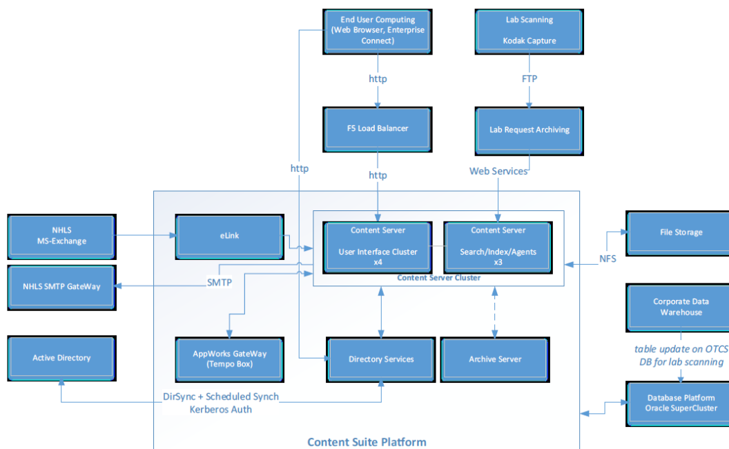
Figure1: ECM Architecture interfaces
