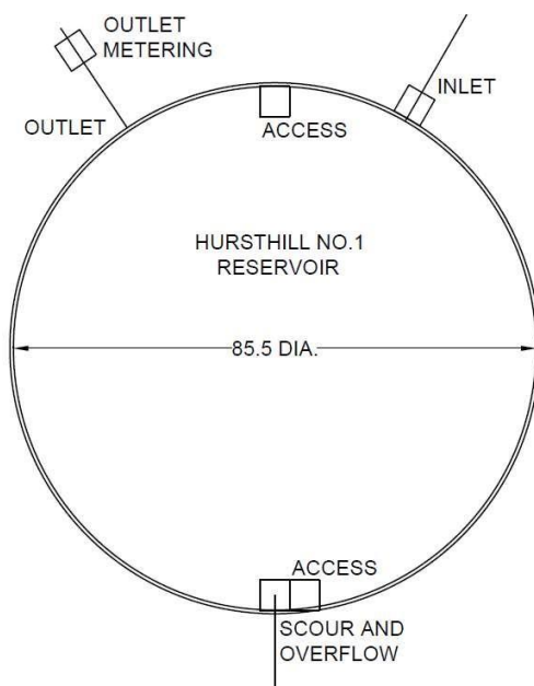
Figure 1: Hursthill Reservoir #1 Schematic Layout
