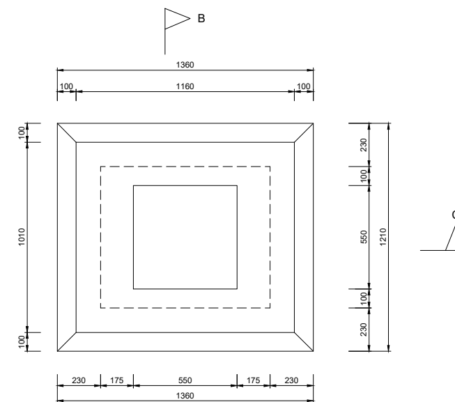
ROOF PLAN SCALE: 12.5
