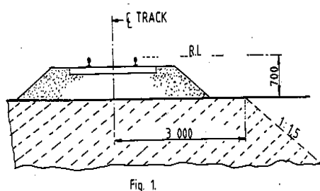
Formation level
