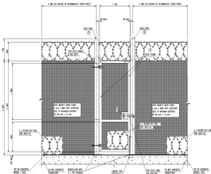
INSIDE ELEVATION OF PEDESTRIAN GATE
