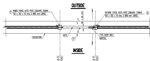
PLAN OF GATE
