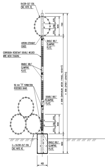
SECTION 01-01
