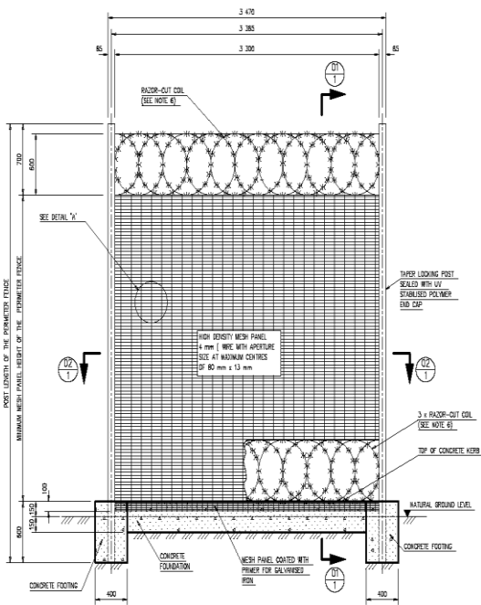
ANTI-INTRUDER FENCING SYSTEM TYPICAL ELEVATION
