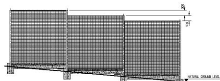
1 PANEL STEP ELEVATION
