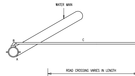
ELEVATION CONNECTION TYPE 6
