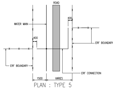
DOUBLE ERF CONNECTION TO BOTH SIDES TYPE 5
