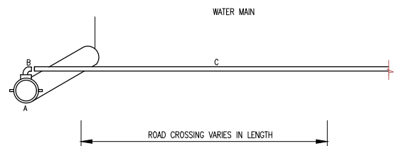
ELEVATION ERF CONNECTION TYPE 7
